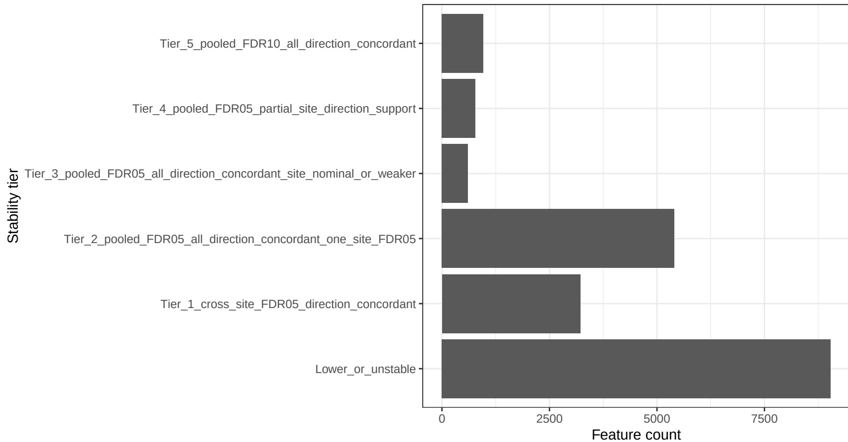
GSE211567 site-aware feature stability tiers
