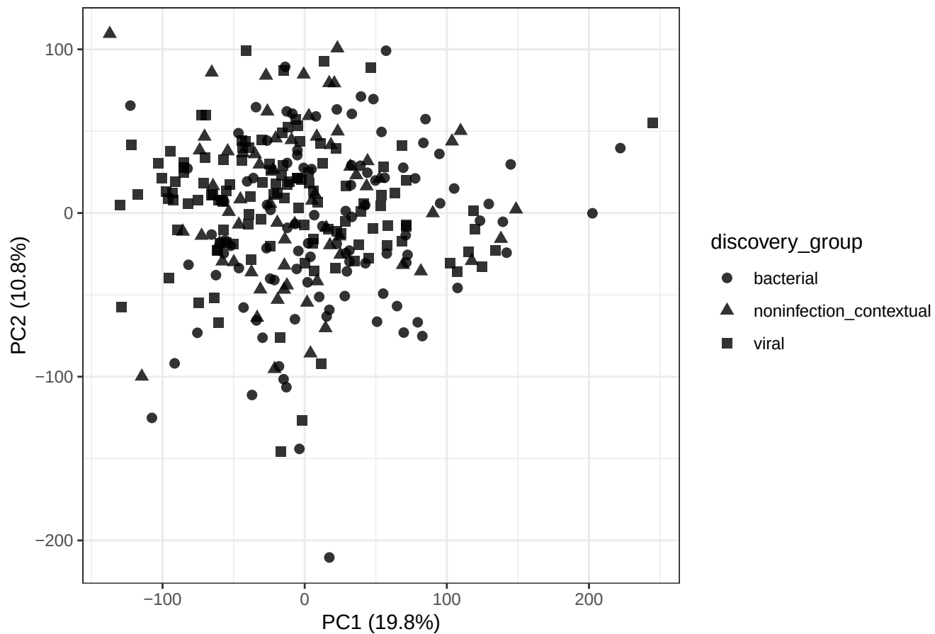
GSE211567 locked samples: PCA by discovery group
