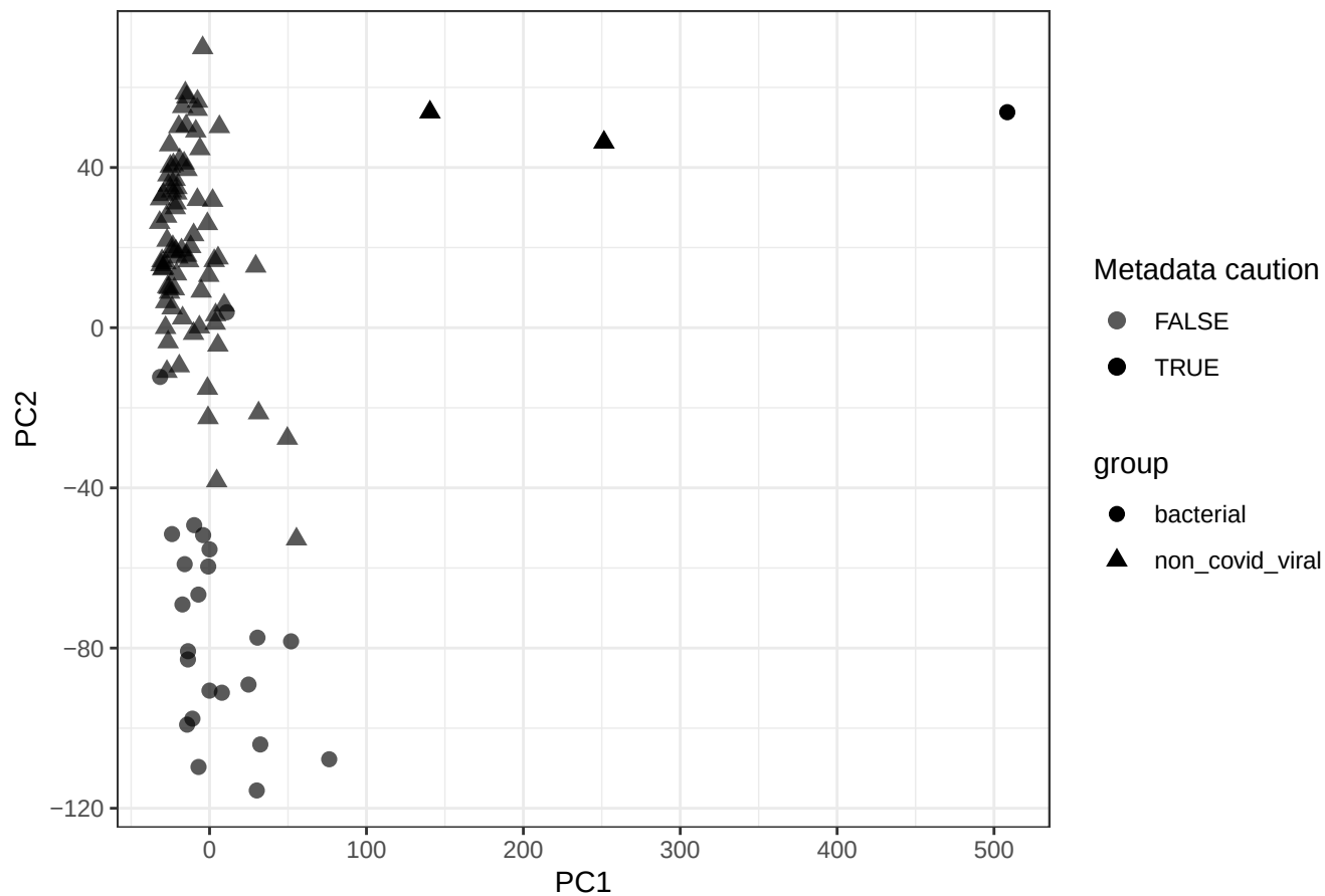
GSE161731 technical rehearsal: PCA with metadata—caution samples highlighted
