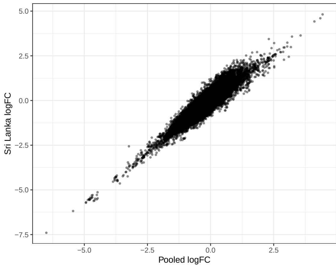
GSE211567_logFC_scatter_pooled_vs_Sri_Lanka
