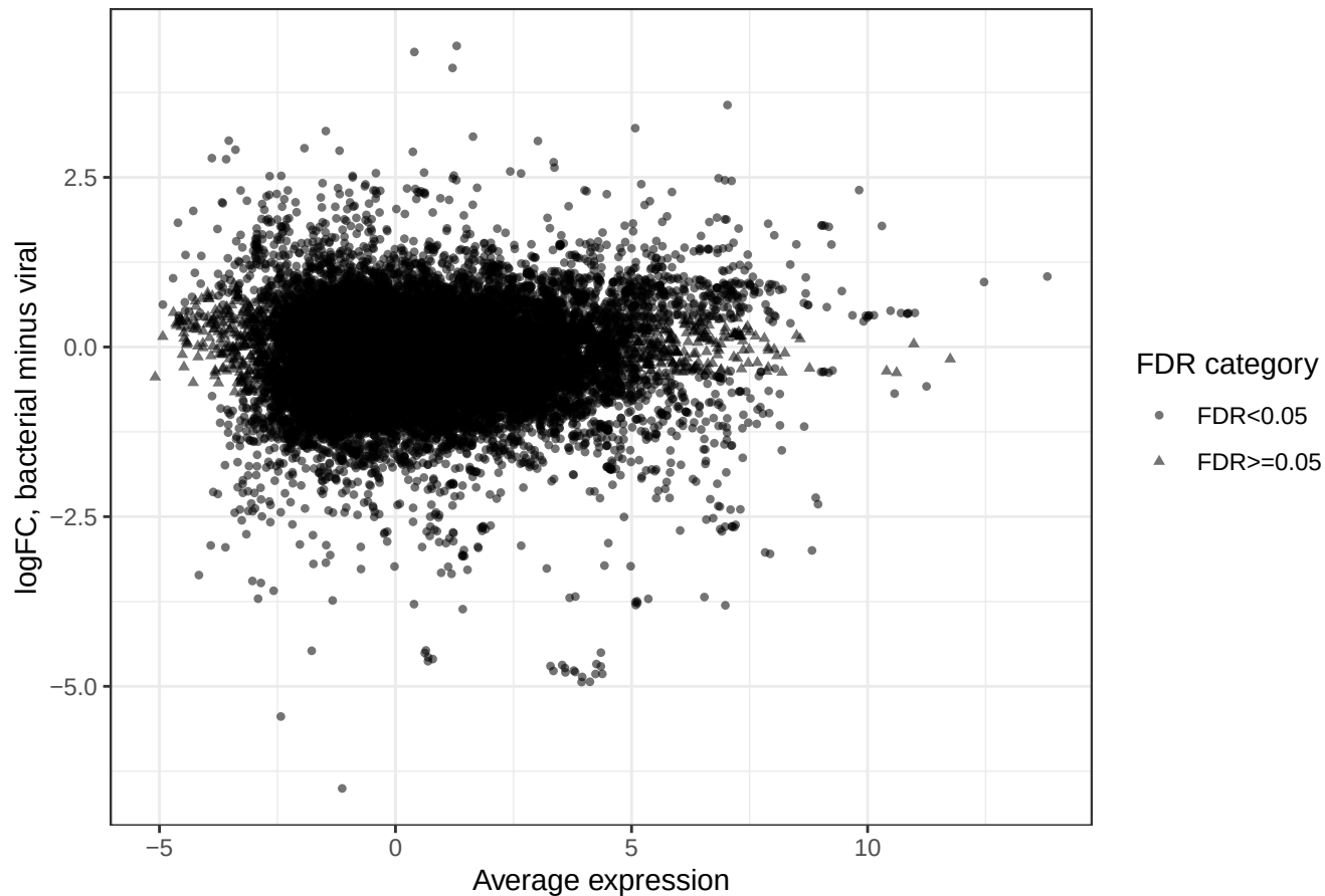
GSE211567 primary limma model: MA-style plot
