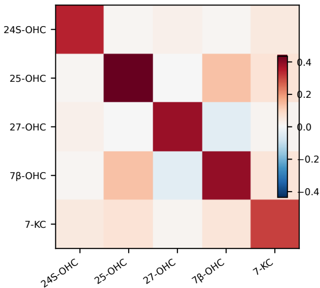
C OAS-shrunk control-baseline covariance
