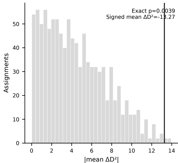
D Exact whole-subject A/B swap reference
