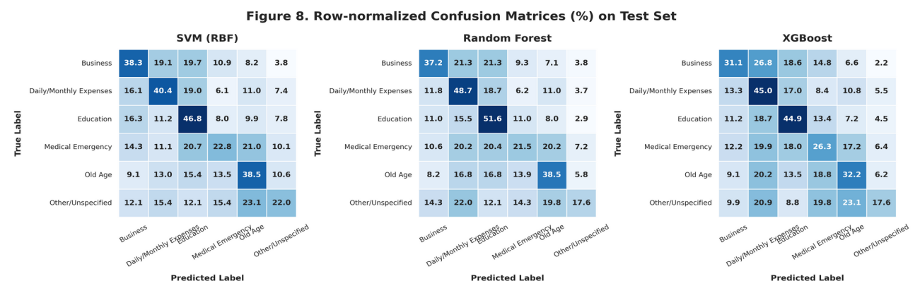
Figure 8. Confusion matrices — SVM, Random Forest, XGBoost (test set)
