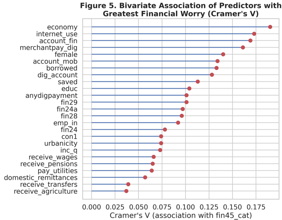
Figure 5. Bivariate association ranking (Cramer's V)
