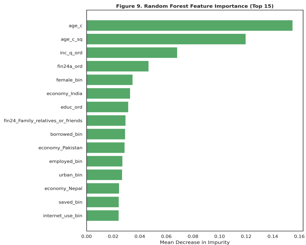
Figure 9. Random Forest feature importance (top 15)
