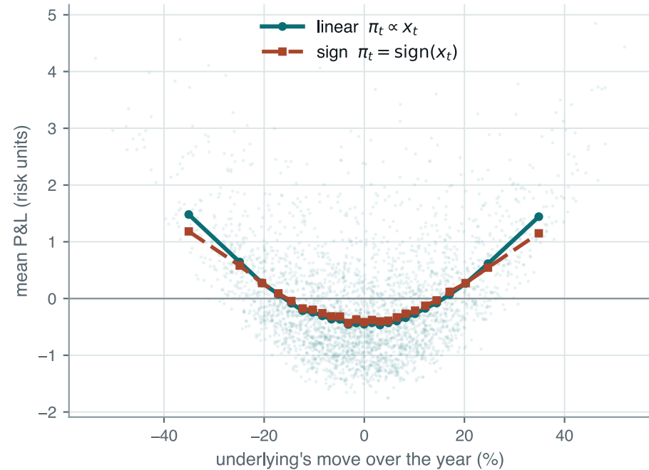
Conditional on the move: a smile
