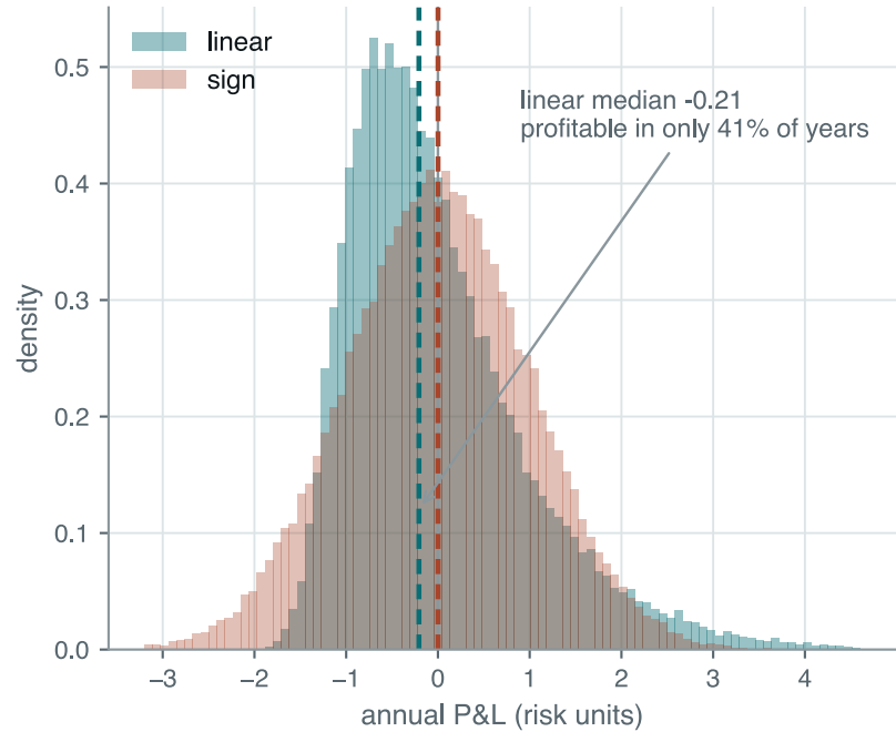
Unconditionally: only the linear rule is skewed
