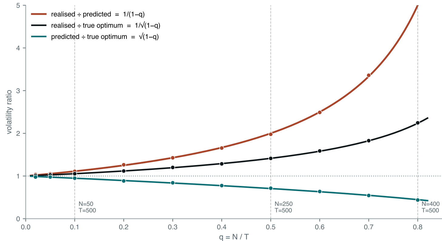
Minimum-variance portfolio risk against the aspect ratio (lines: theory, dots: simulation)
