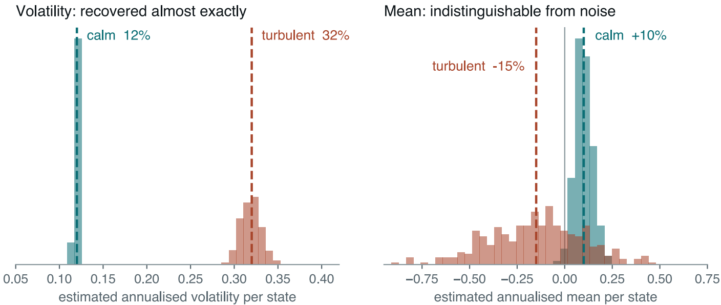
400 simulations, 10 years of daily data, correctly specified K = 2 Gaussian HMM, true parameters known to exist. Volatility ratio recovered with 3.7% relative error; the estimated mean spread has the WRONG SIGN in 16% of samples.
