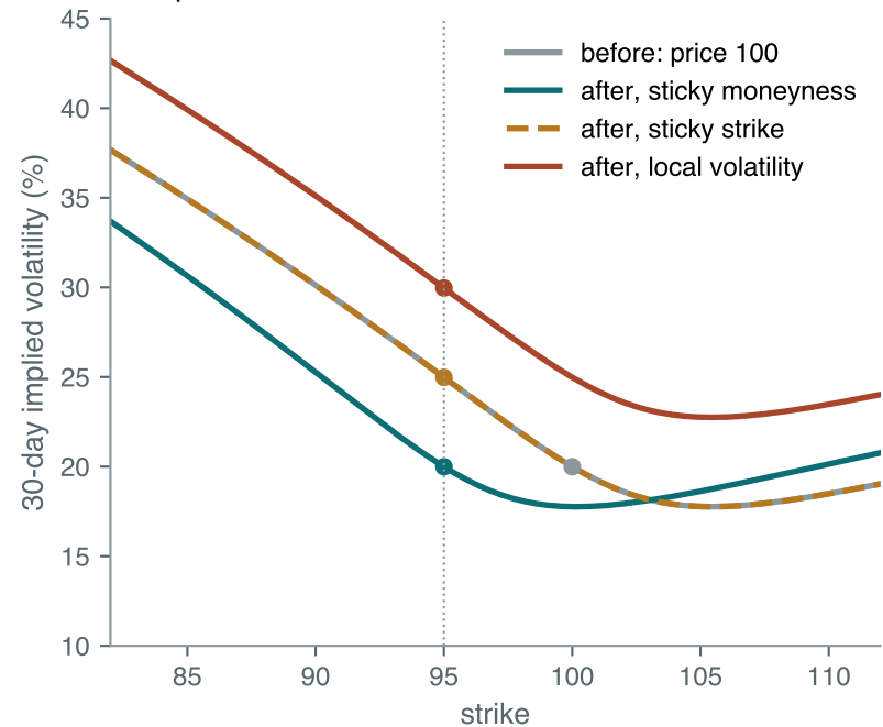
The price falls 5%: three rules
