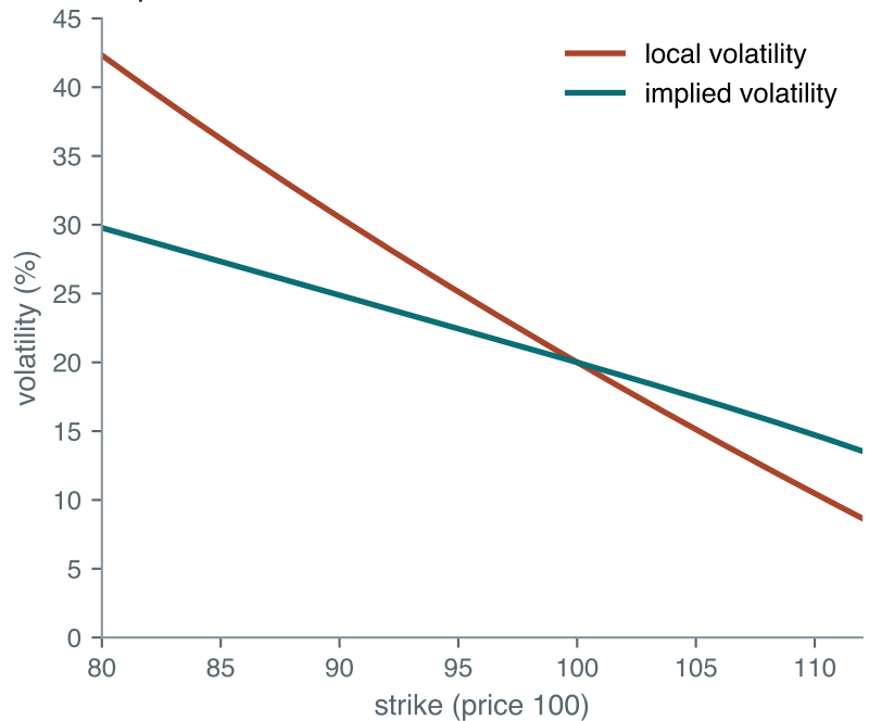
Implied skew is half the local skew
