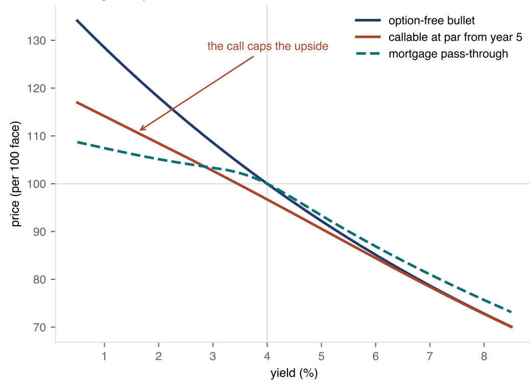
Price against yield
