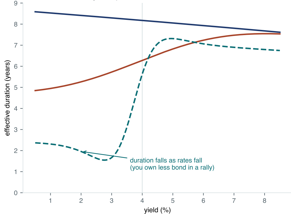
Effective duration against yield
