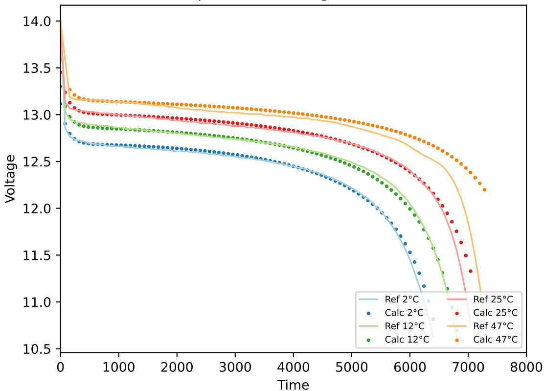
Comparison of Voltage Over Time
