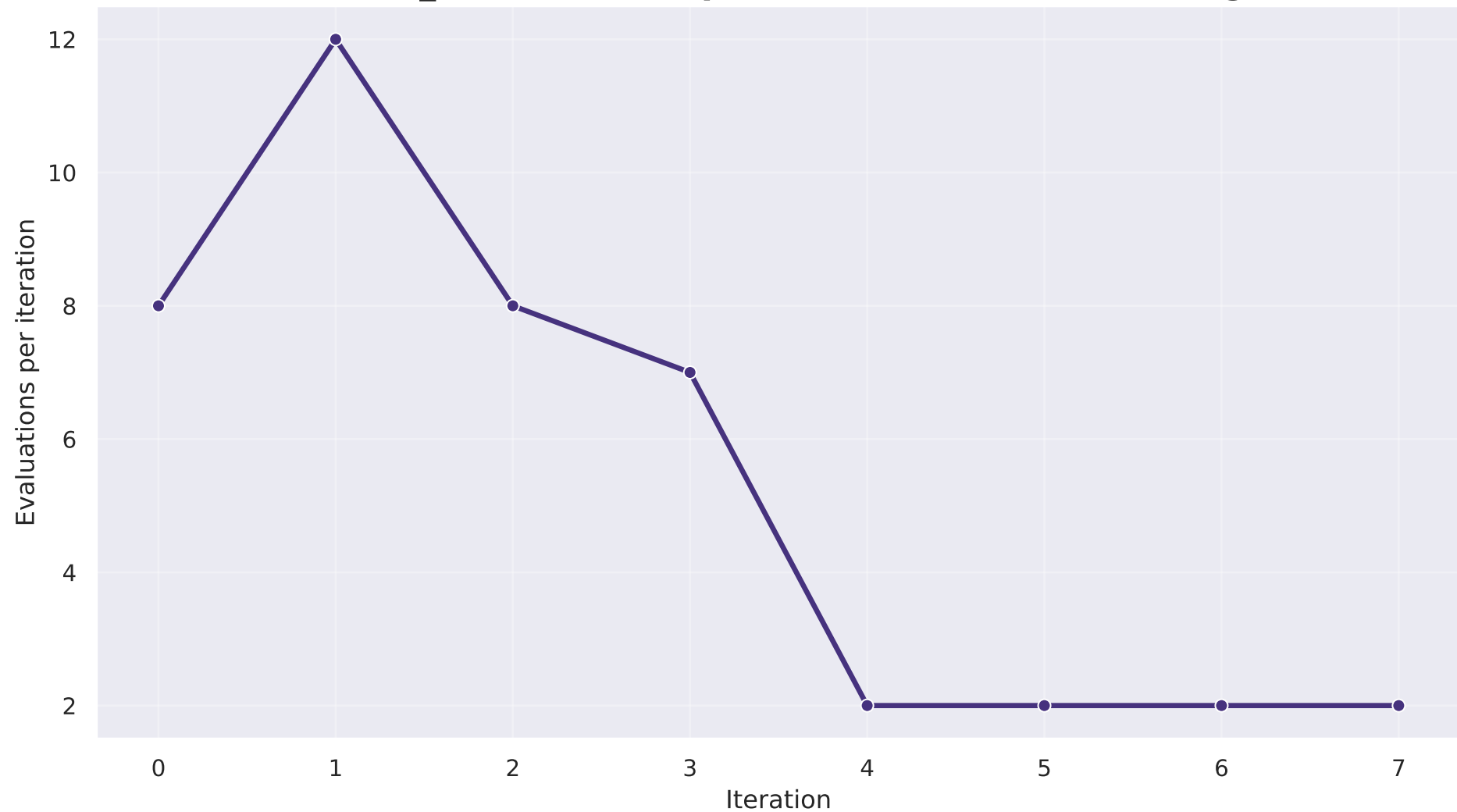
Number of P_n evaluations per iteration of the Brent algorithm
