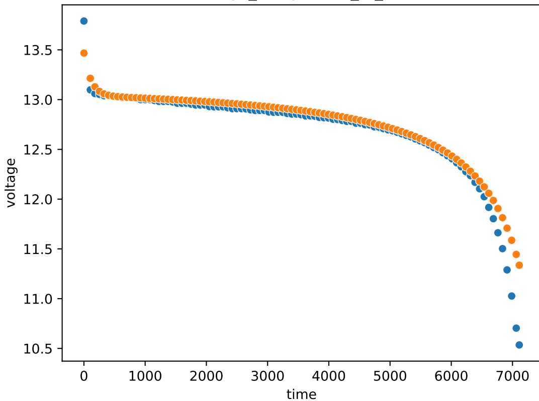
voltage_comparison_at_25C
