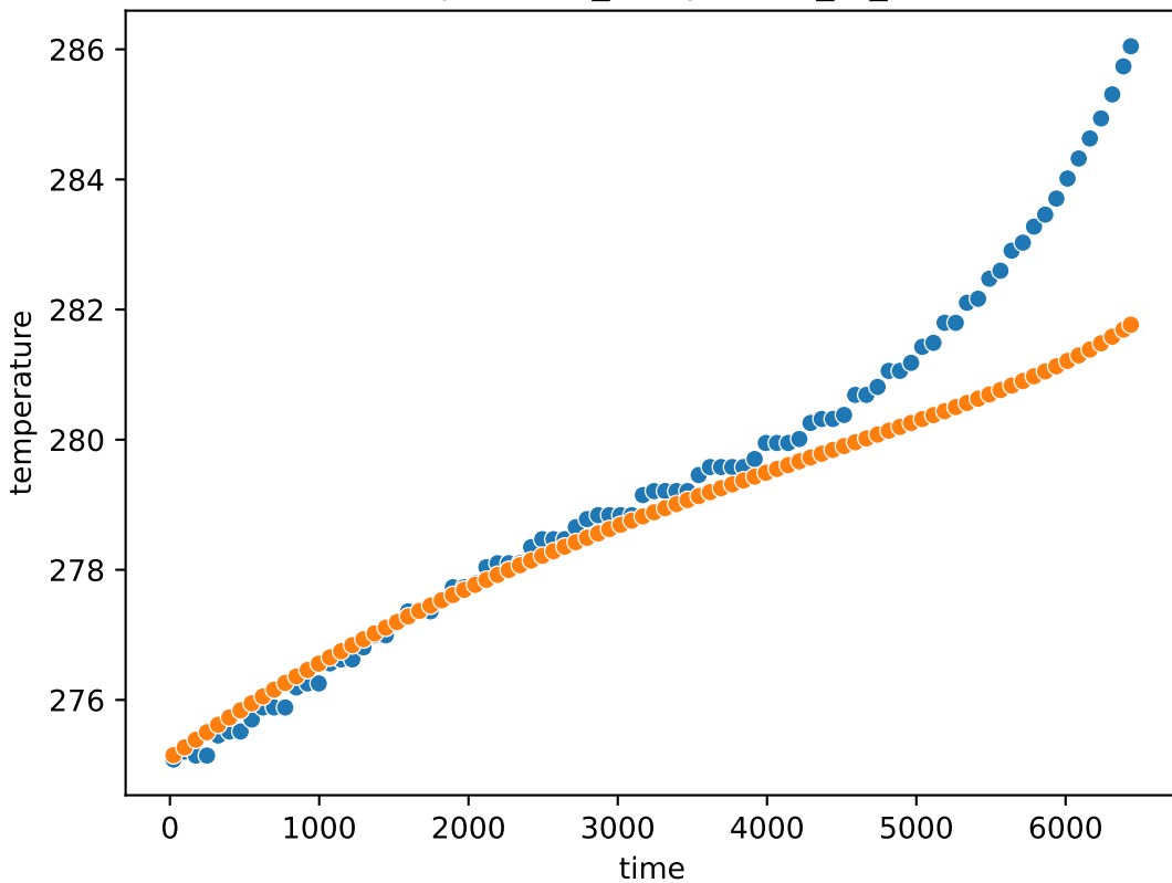
temperature_comparison_at_2C
