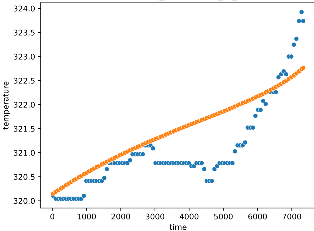
temperature_comparison_at_47C
