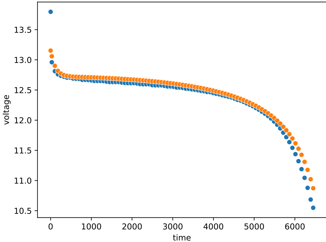
voltage_comparison_at_2C
