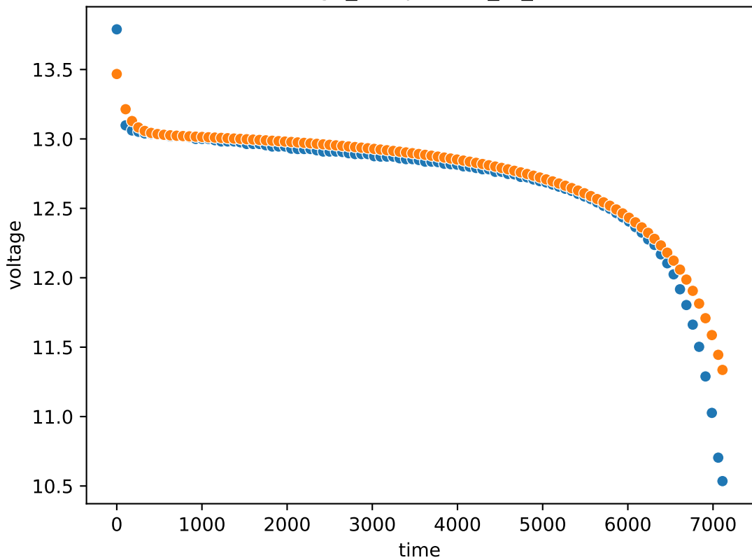
voltage_comparison_at_25C
