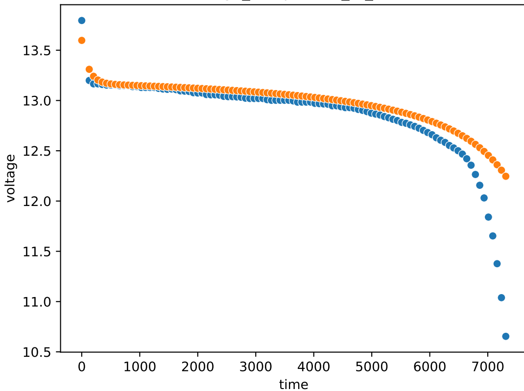
voltage_comparison_at_47C
