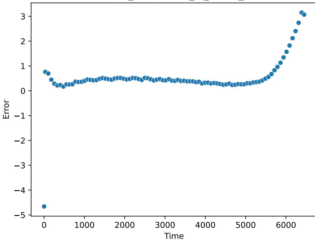
voltage_comparison_at_2C-err_rel
