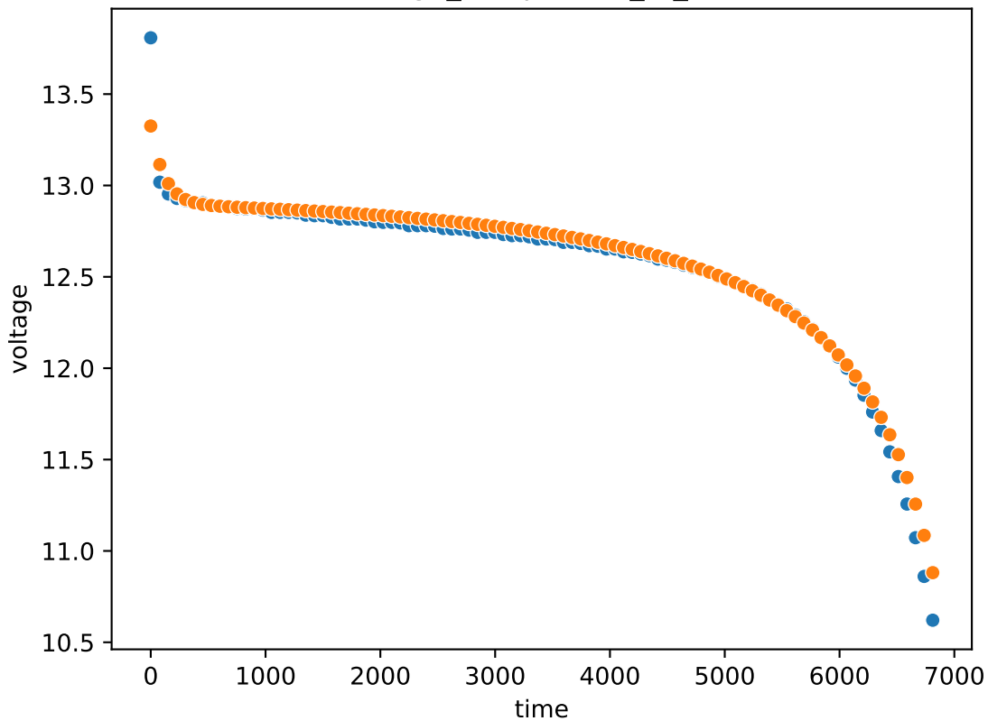
voltage_comparison_at_12C
