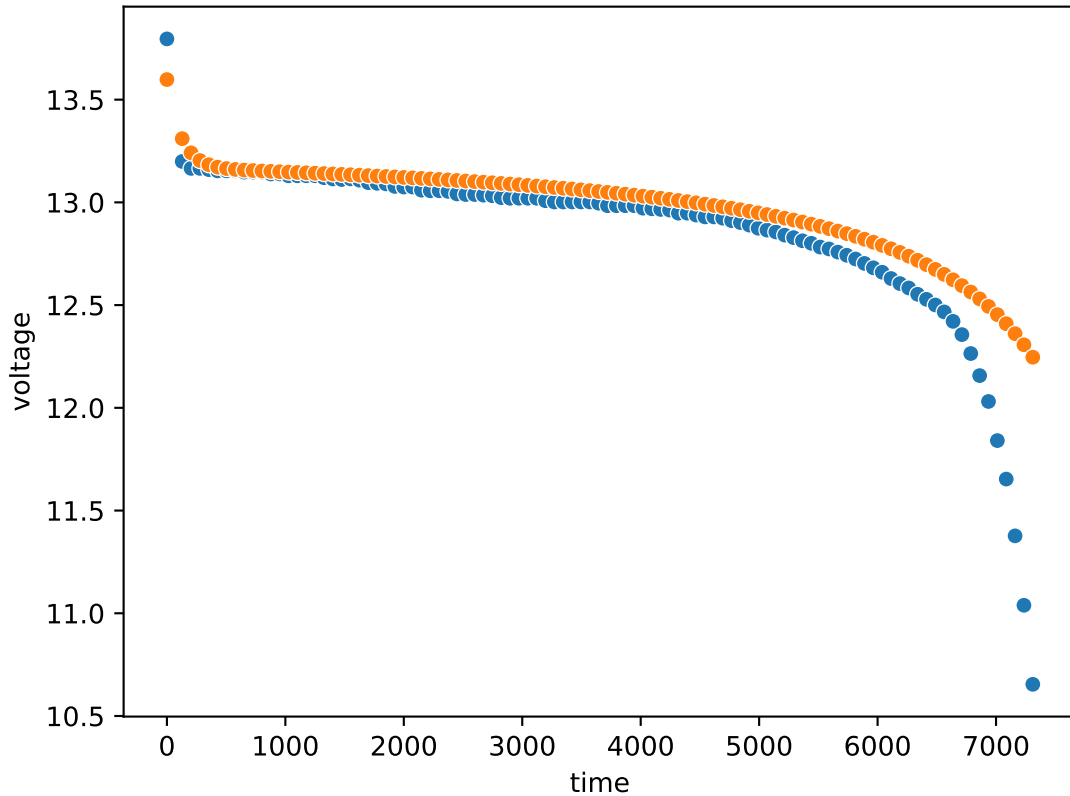
voltage_comparison_at_47C
