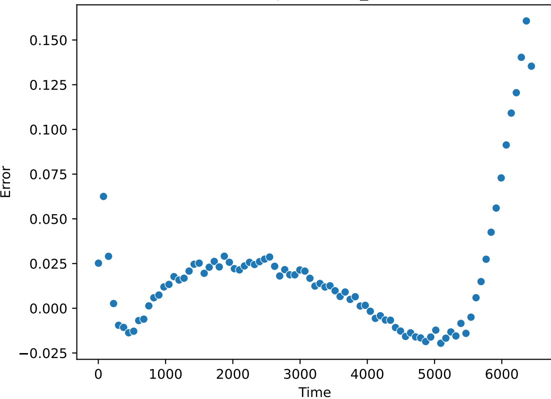
VoltageError-err_abs
