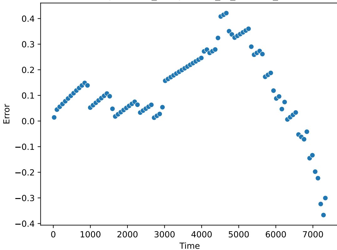
temperature_comparison_at_47C-err_rel
