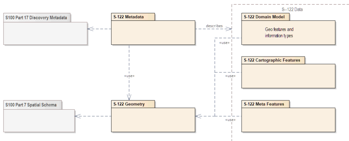
Figure 4-2 — S-122 Data model overview
