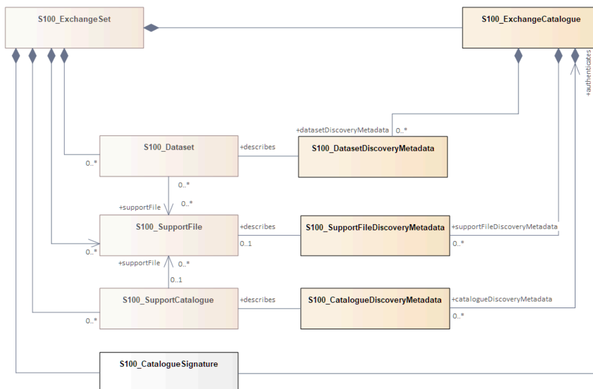
Figure 13-1 — Components and associated metadata for the S-122 exchange set (S-100 Figure 17-2)
