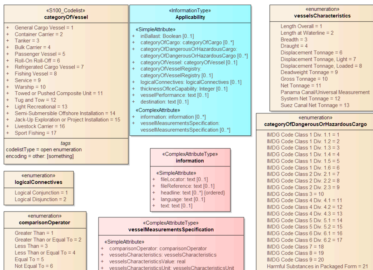
Figure 4-12 — Vessel subsets characterised by cargo, dimensions and capabilities
