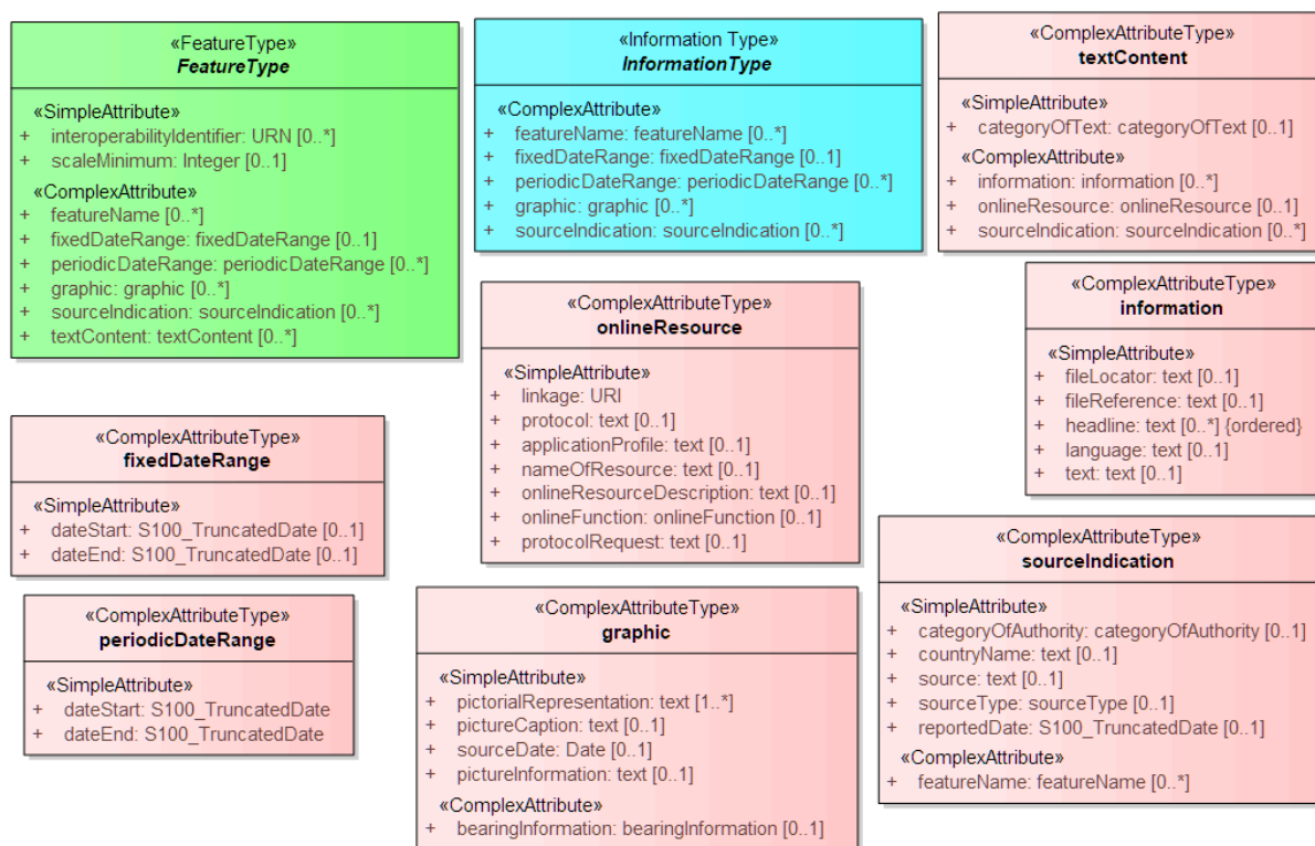
Figure 4-3 — Base classes in S-122
