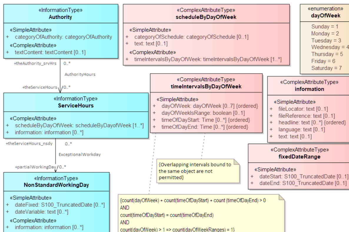
Figure 4-10 — Working times and schedules
