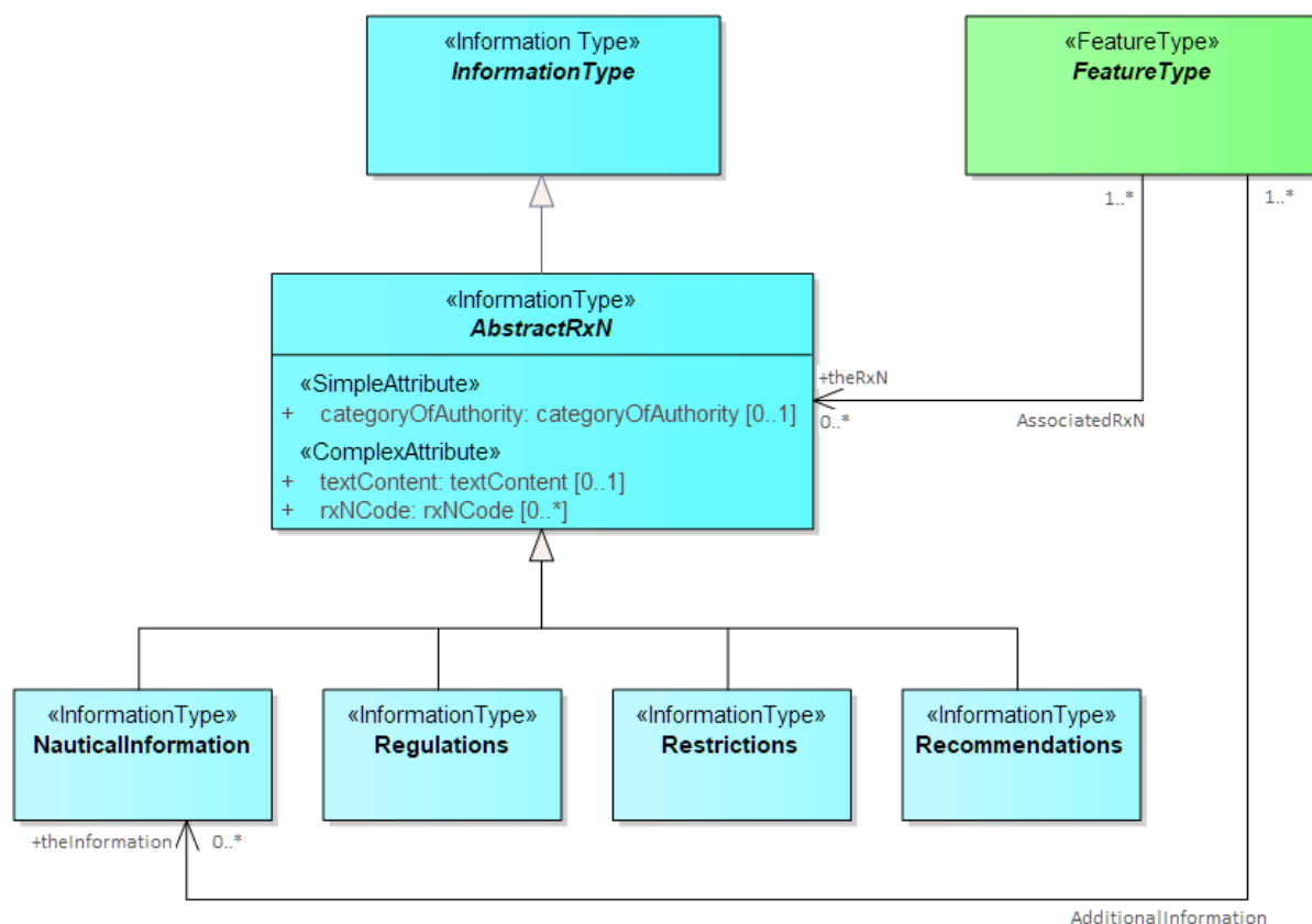
Figure 4-16 — Attachment of uncategorizable information to any feature type
