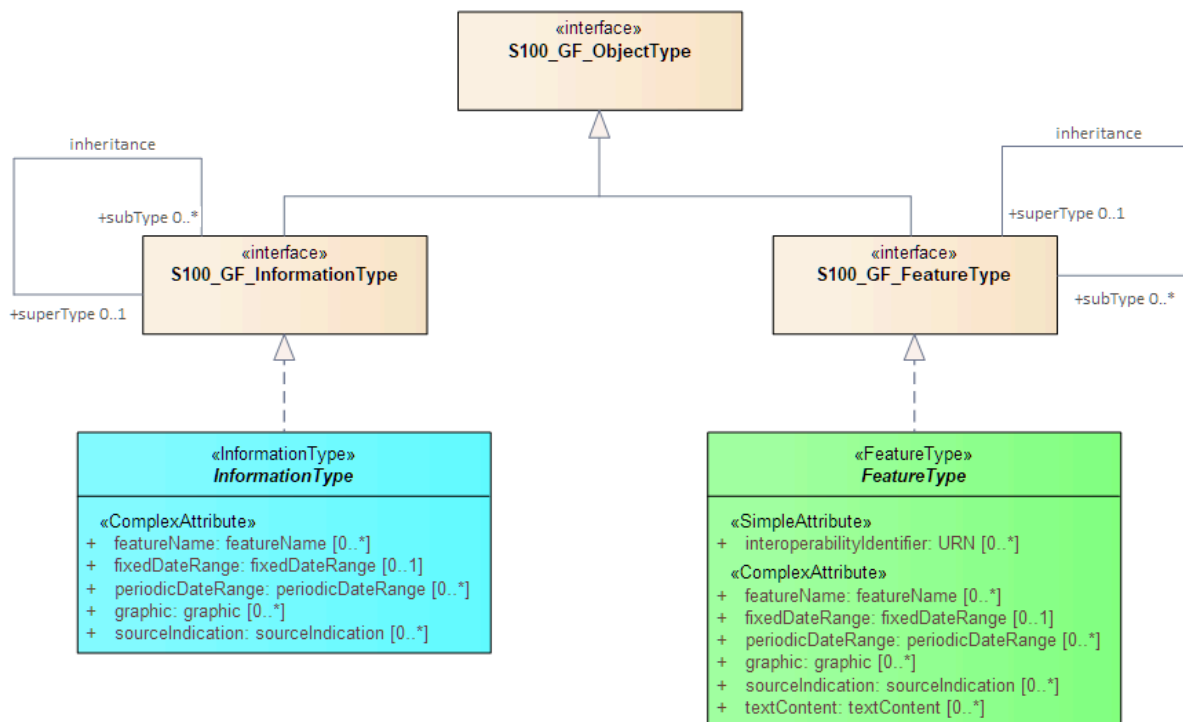
Figure 4-1 — Realizations from the S-100 General Feature Model
