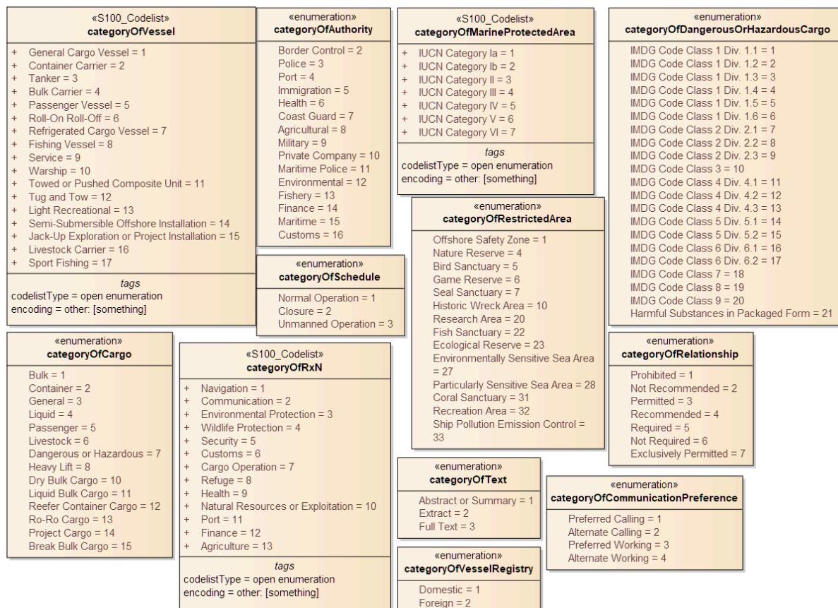
Figure 4-14 — Category enumerations and codelists
