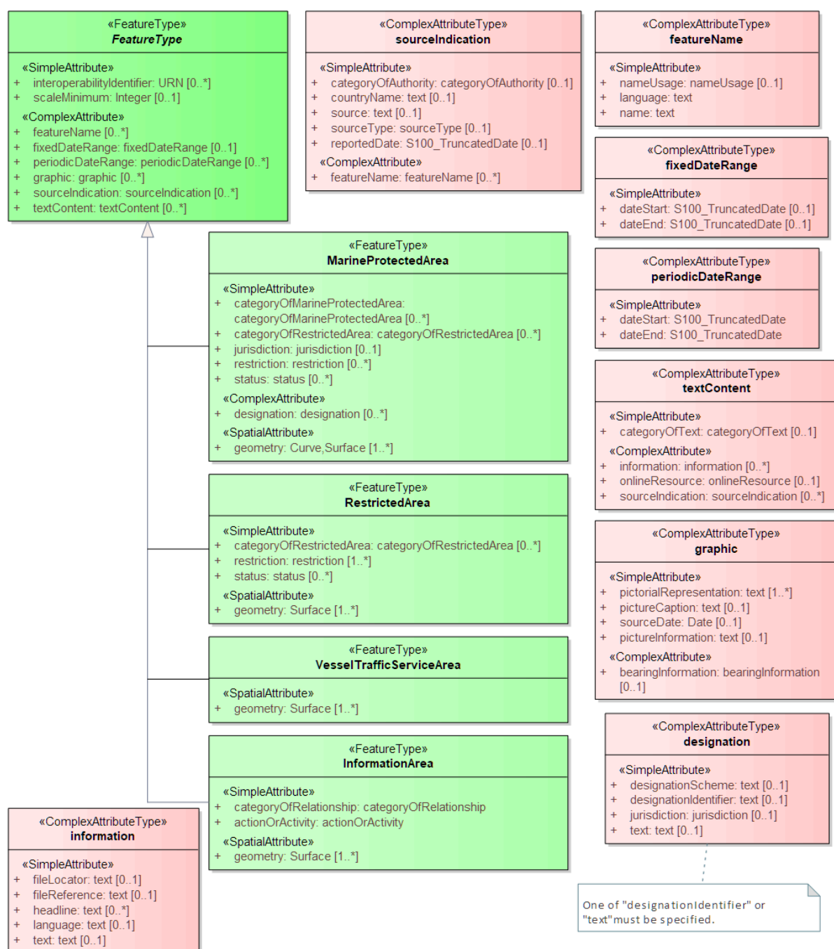
Figure 4-4 — Overview of S-122 Feature Types
