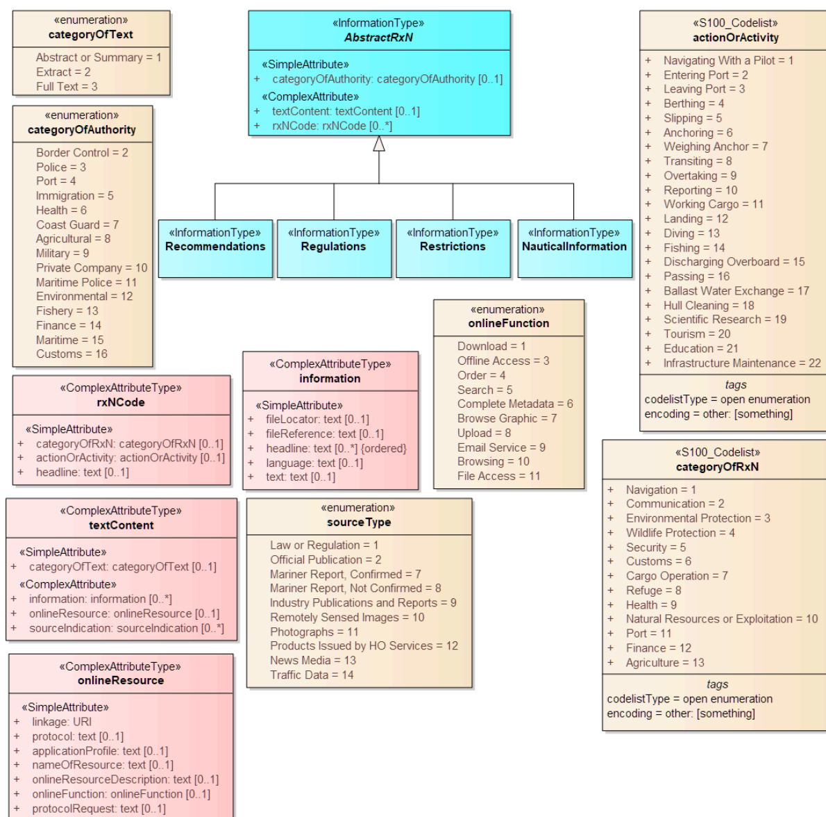
Figure 4-7 — Regulations and other information types for primarily textual information
