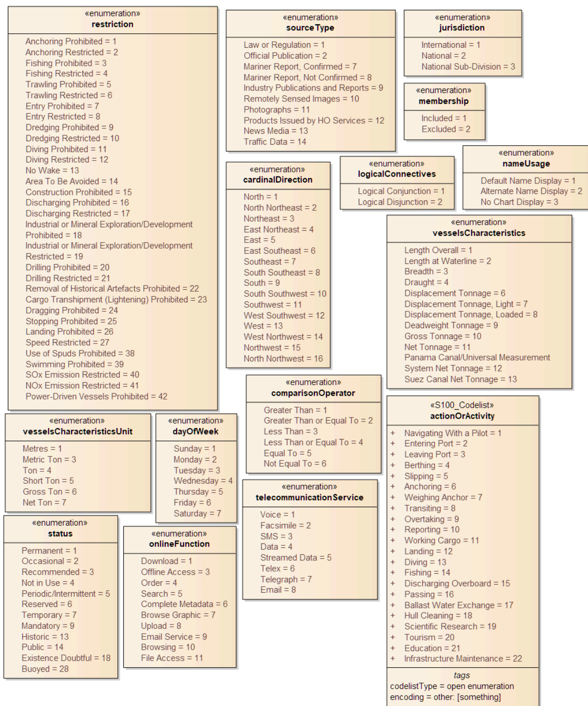
Figure 4-15 — Other enumerations and codelists
