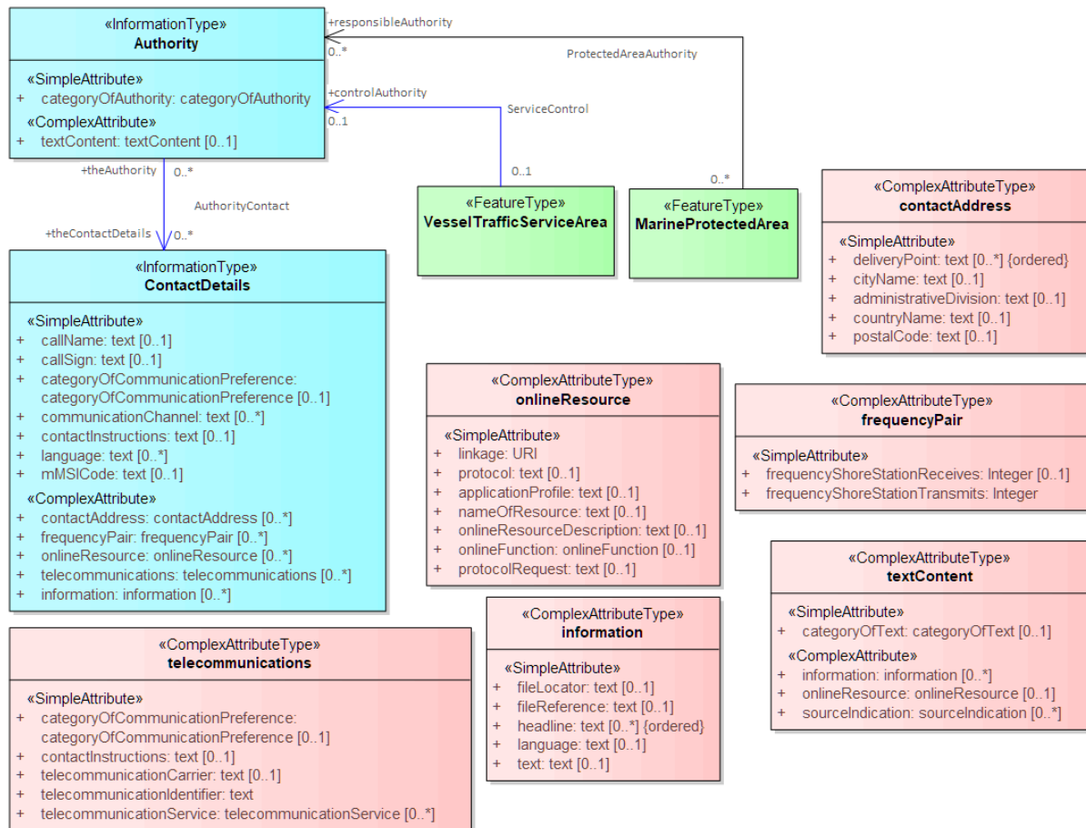
Figure 4-8 — Authorities and their contact information
