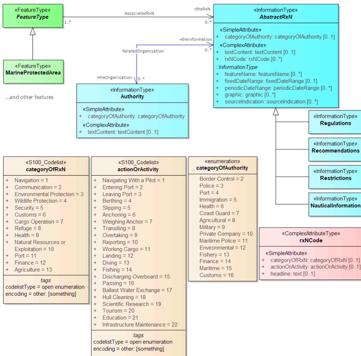
Figure 4-11 — Regulations, etc., relevant to specific features
