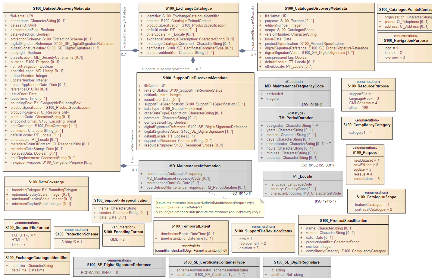
Figure 14-2 — Details of exchange set catalogue classes. (Derived from S-100 Figure 17-7.)
