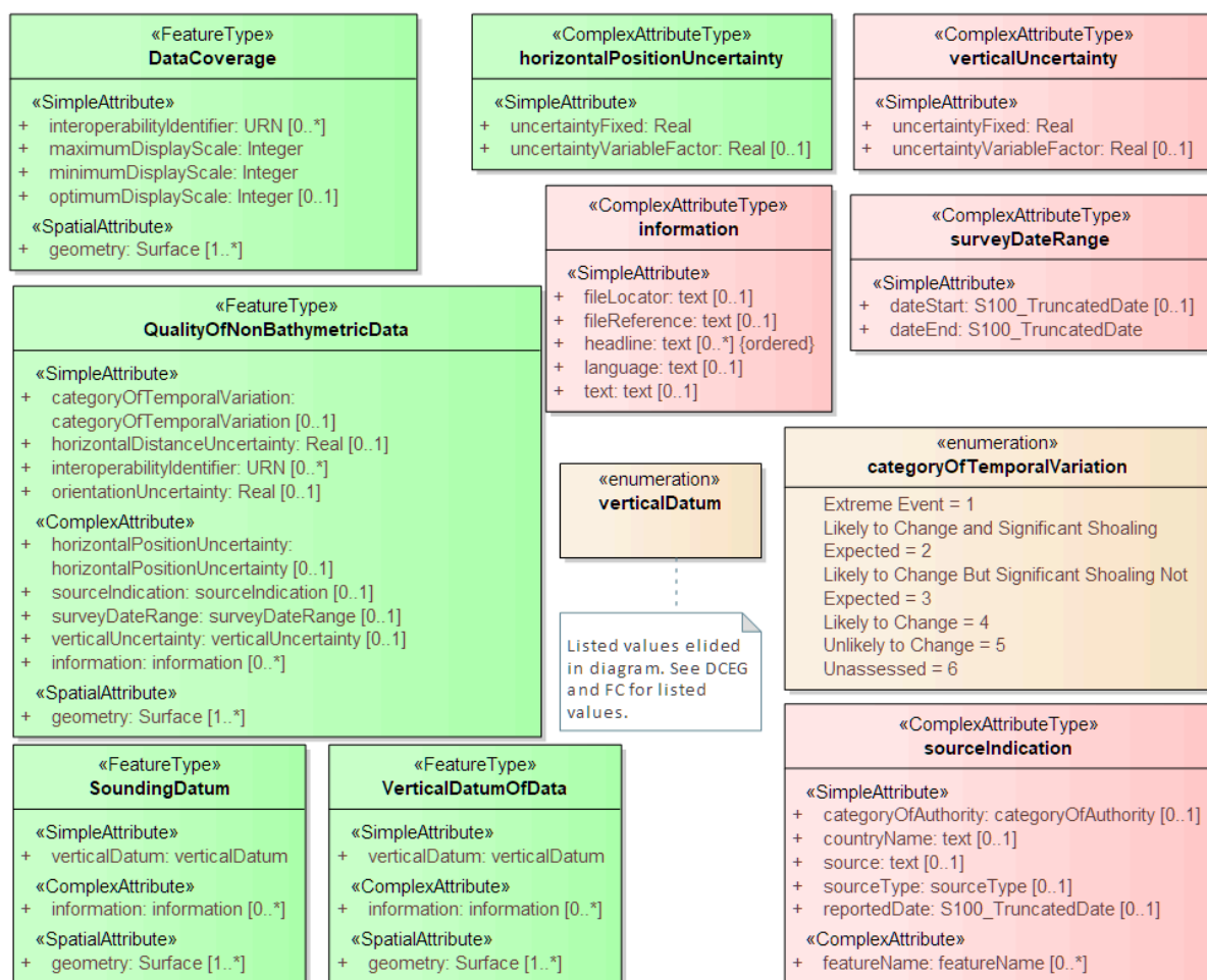
Figure 4-21 — Meta-feature classes
