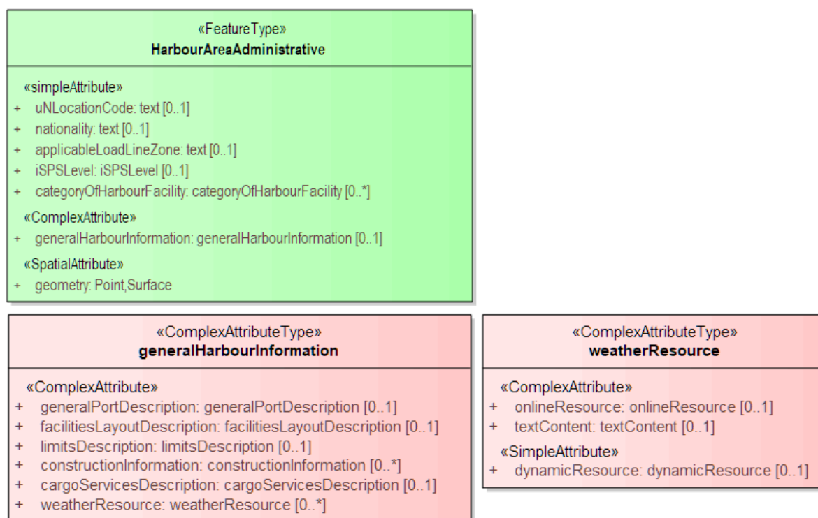
Figure 5-1 — Complex attribute
