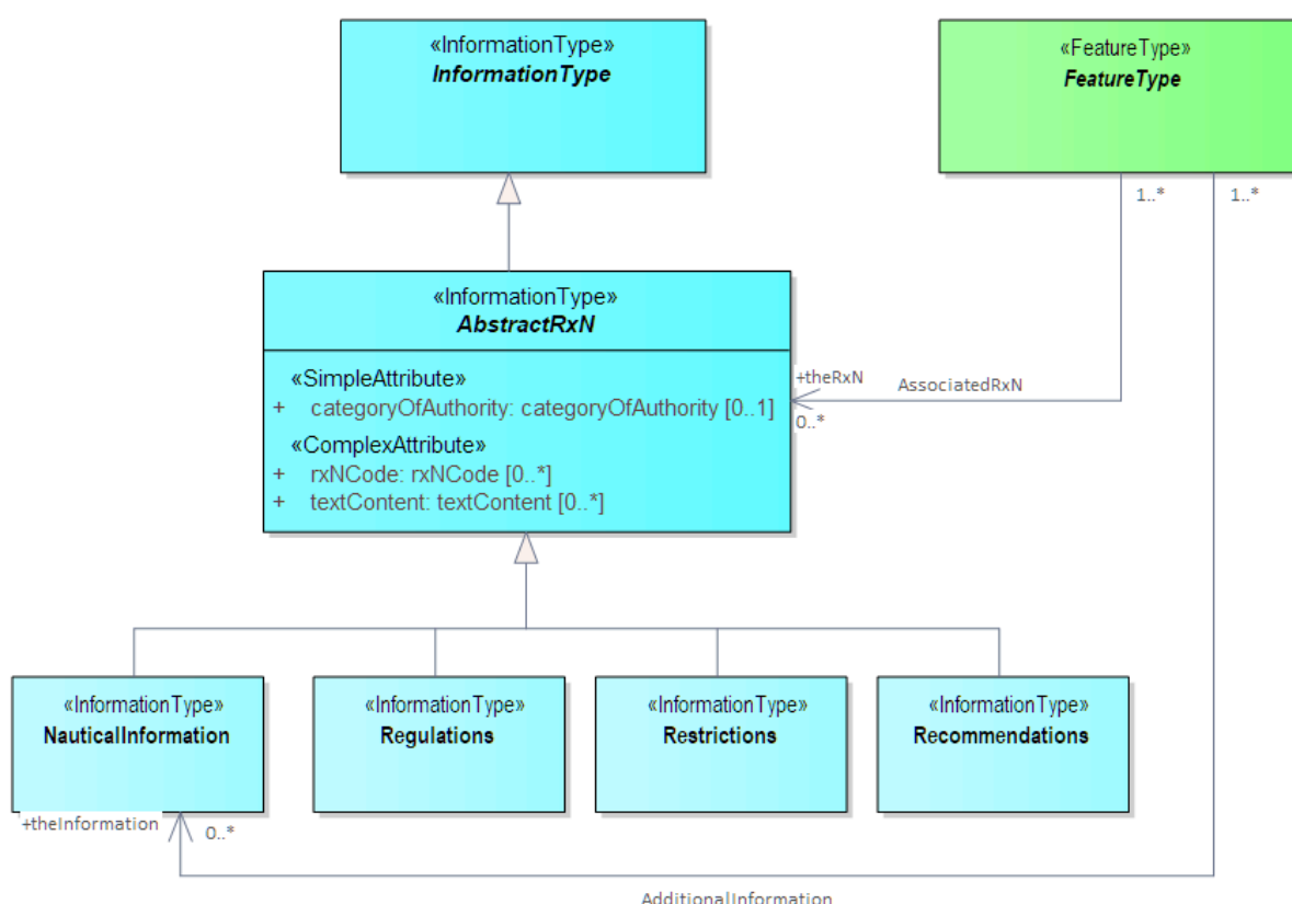
Figure 4-18 — Attachment of uncategorizable information to any feature or information type
