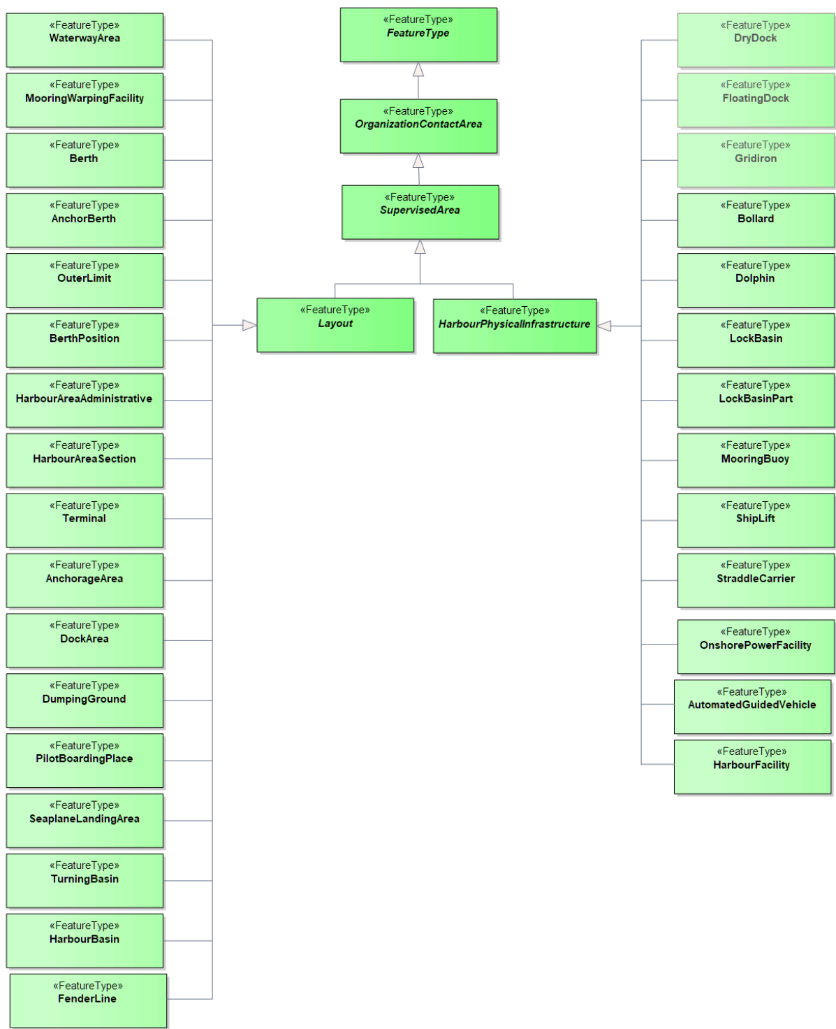
Figure 4-3 — Overview of S-131 domain feature classes
