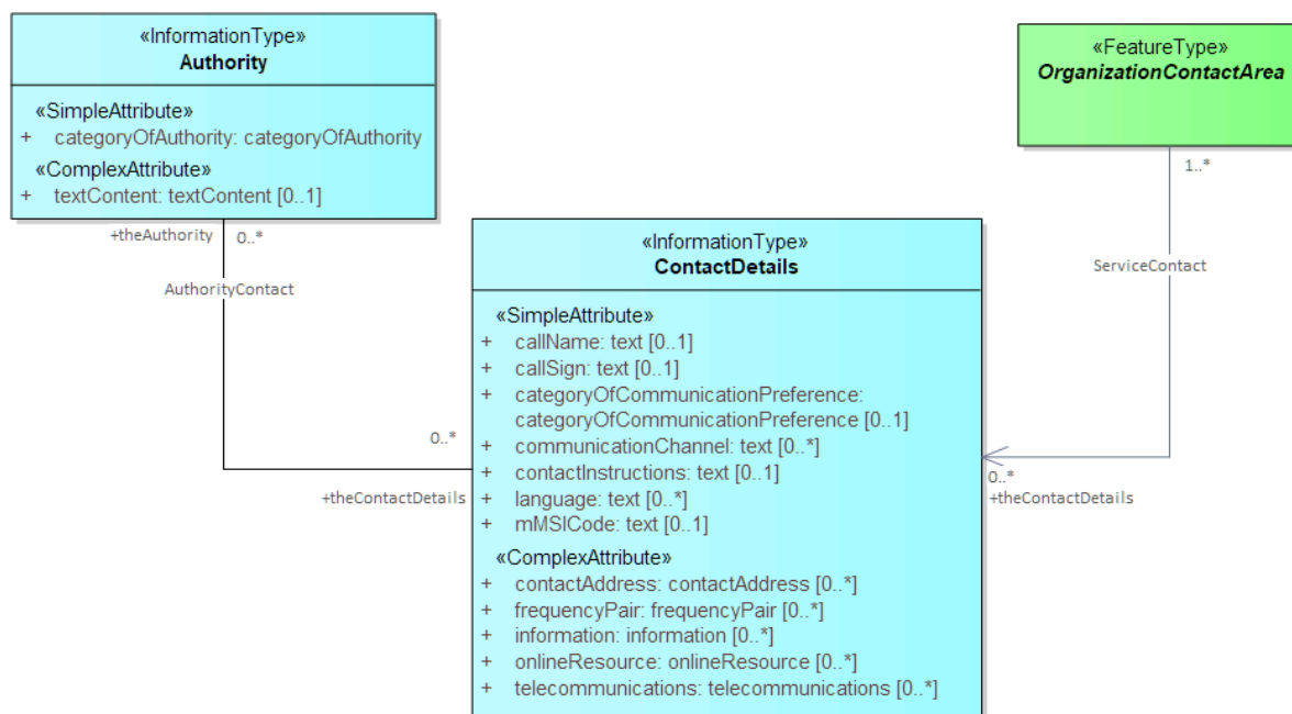
Figure 4-13 — Associations to contact information
