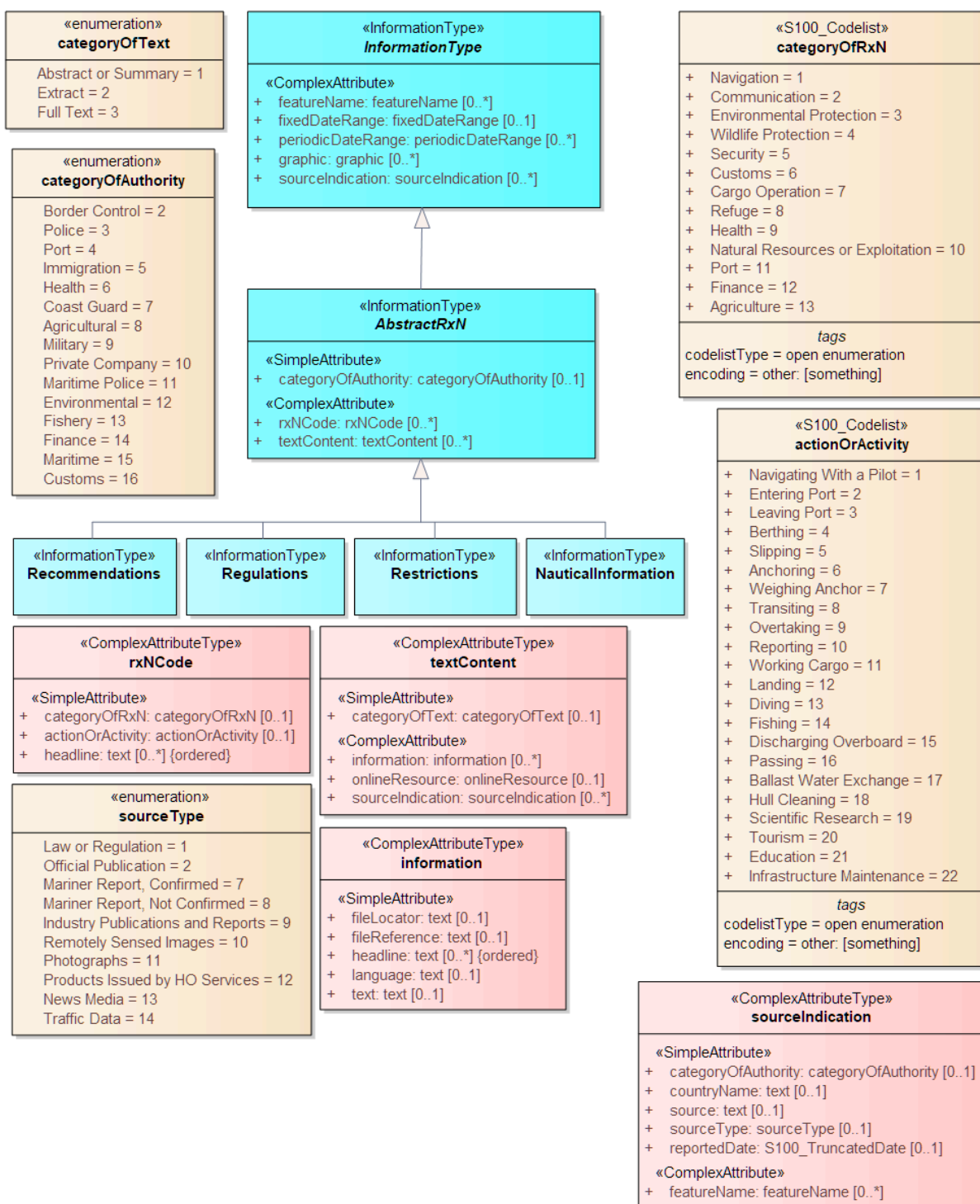
Figure 4-11 — Regulations and other information types for primarily textual information
