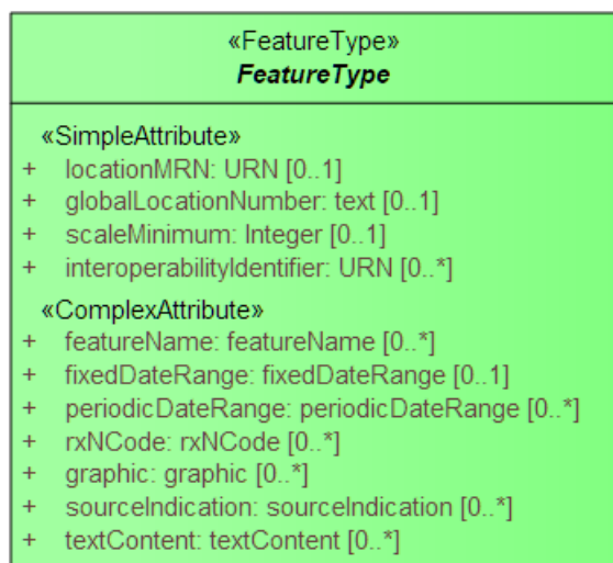
Figure 4-5 — The root class FeatureType
