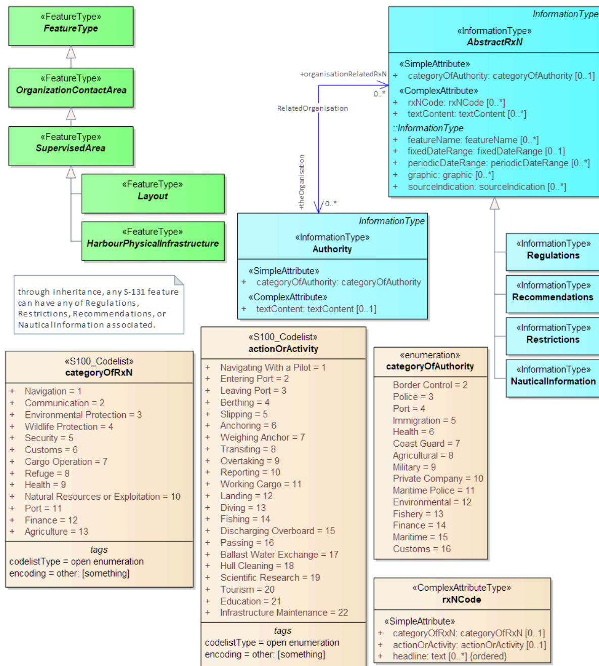
Figure 4-15 — Regulations, etc., applying to specific features
