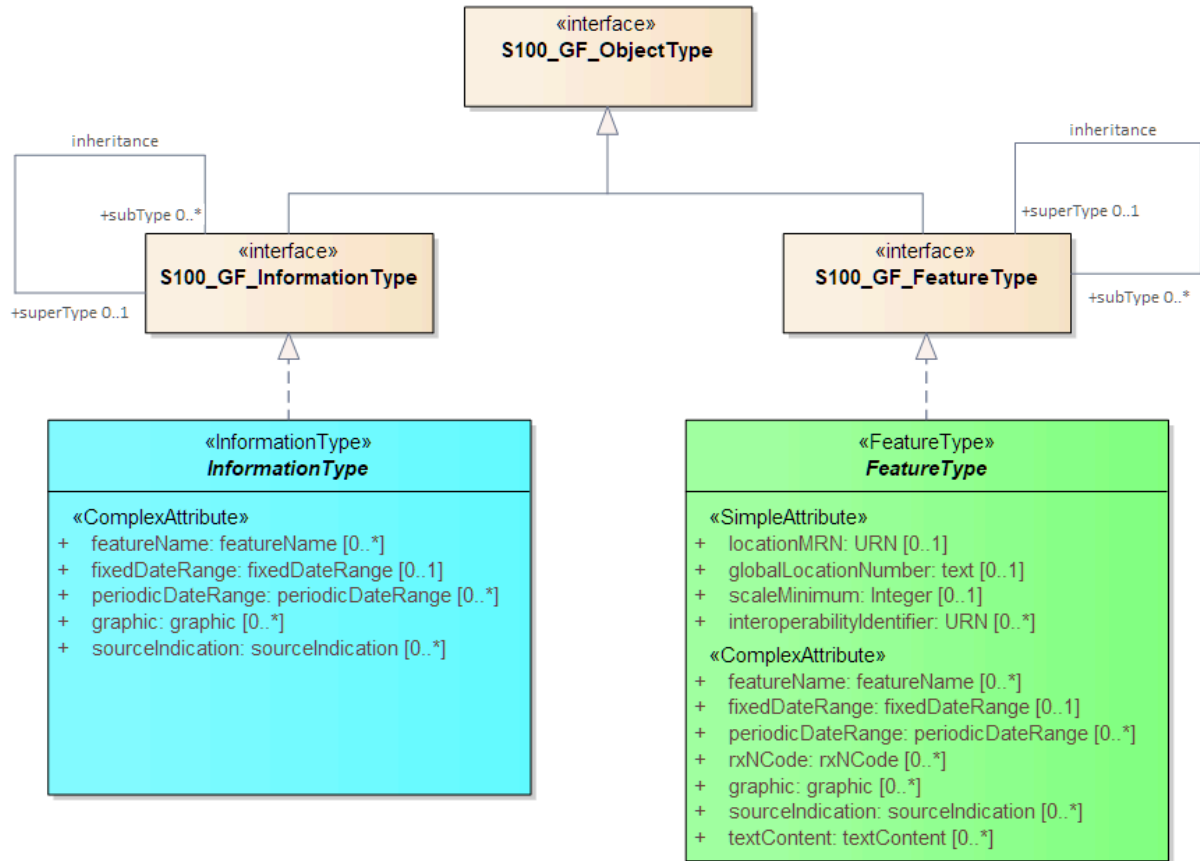
Figure 4-1 — Realizations from the S-100 General Feature Model
