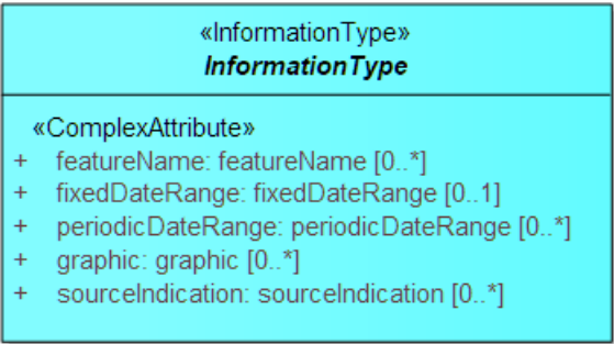
Figure 4-6 — The root class InformationType
