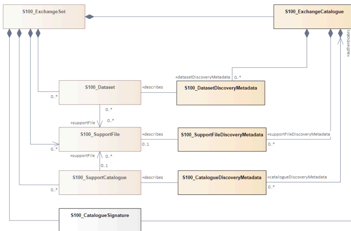
Figure 13-1 — Components and associated metadata for the S-131 exchange set (S-100 Figure 17-2)
