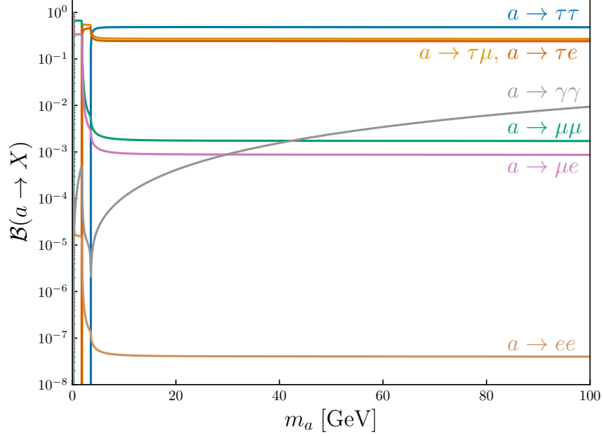
Figure 5.1: ALP branching fraction assuming a democratic lepton coupling matrix (and all other couplings zero). The ALP will decay to at least one \tau roughly 99.7% of the time.
