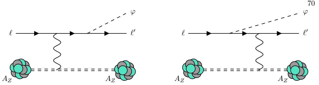
Figure 4.1: Relevant Feynman diagrams for the process \ell A_Z \rightarrow \ell' A_Z \phi via photon exchange.
