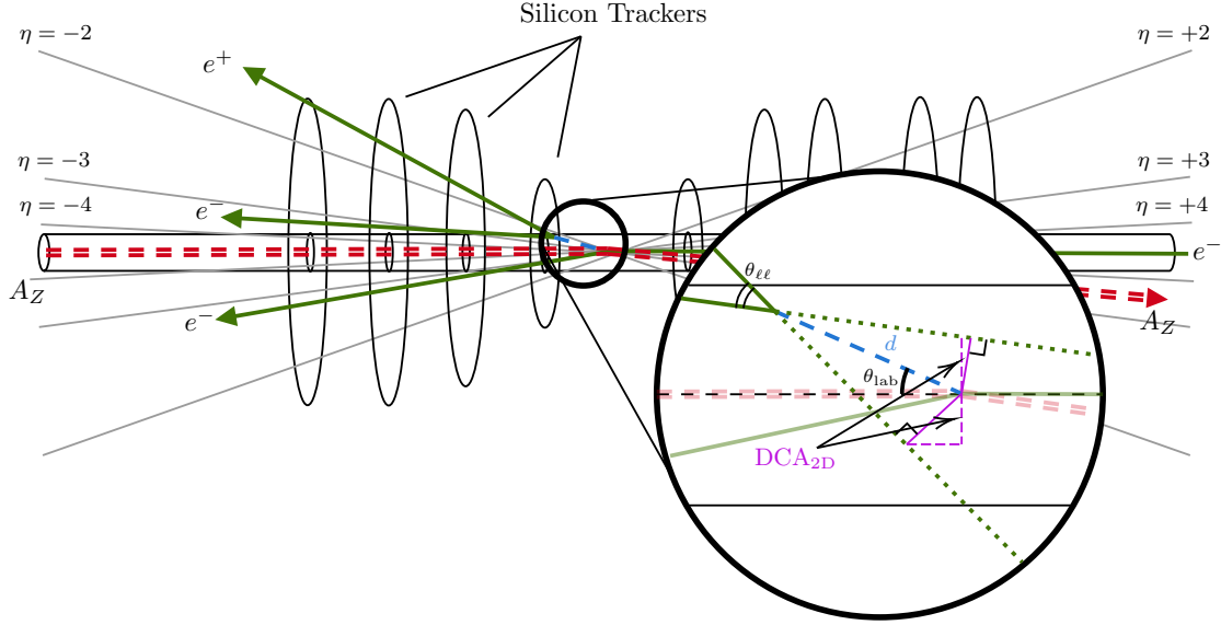
Figure 6.2: A schematic representation of the displaced process under consideration, including a diagram the transverse distance-of-closest-approach ( \text{DCA}_{2\text{D}} ) for the final-state decay e^+e^- products of a vector boson with displacement d at the EIC. The tracks of the electrons and positrons in the final-state are shown as solid green lines, and the reconstructed tracks of the e^+e^- decay products from the dark boson are shown as dashed green lines. The distance-of-closest-approach for each decay product is depicted as a solid magenta line, and its transverse component (the \text{DCA}_{2\text{D}} ) is depicted as a vertical dashed magenta line. The size of the beam-pipe and placement of the silicon tracker is reproduced from Ref. [149]. In order to ensure each track can be reconstructed with the desired precision, we require that the vector boson decays before the first silicon tracker, which is placed 25 cm from the interaction point.
