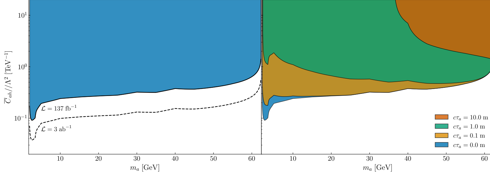
CMS Limit and Projection for Promptly Decaying ALPs
