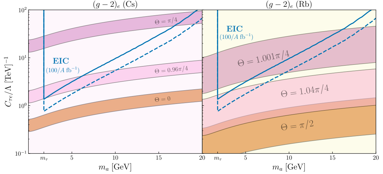
Figure 5.8: Expected limits on C_{\tau e}/\Lambda from the EIC, alongside explanations for the electron g-2 anomalies for different PV angles \Theta . The left panel presents 2\sigma explanations for the anomaly obtained from using \alpha(\text{Cs}) , and the right panel presents explanations for the anomaly obtained from using \alpha(\text{Rb}) .
