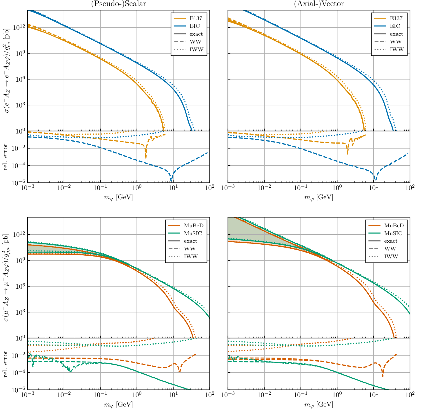
Figure 4.4: Comparisons between exact (solid) and approximate (“WW,” dashed and “IWW,” dotted) cross-sections, along with relative errors (bottom of each plot), for some lepton-nucleus collisions. The plots on the top compare the approximate and exact cross-sections for the electron-nucleus collisions at E137 and the EIC, whereas the plots on the bottom compare the approximate and exact cross-sections for the muon-nucleus collisions at the hypothetical 1 TeV MuBeD and MuSIC (defined in the text). The plots on the left compare the results for (pseudo)-scalars, while the plots on the right compare the results for (axial)-vectors.
