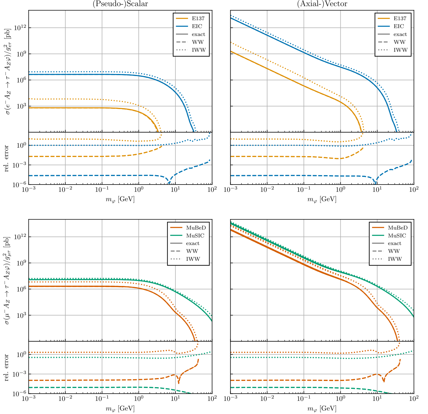
Figure 4.5: Comparisons between exact (solid) and approximate (“WW,” dashed and “IWW,” dotted) cross-sections, along with relative errors (bottom of each plot), for some lepton-nucleus collisions. The plots on the top compare the approximate and exact cross-sections for the electron-nucleus collisions at E137 and the EIC, whereas the plots on the bottom compare the approximate and exact cross-sections for the muon-nucleus collisions at the hypothetical 1 TeV MuBeD and MuSIC (defined in the text). The plots on the left compare the results for (pseudo)-scalars, while the plots on the right compare the results for (axial)-vectors.
