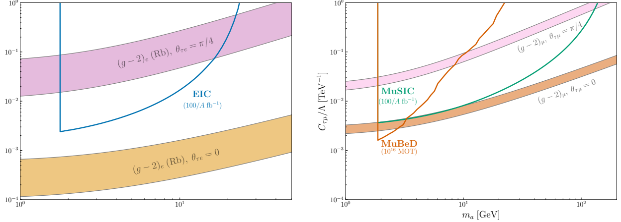
Figure 4.11: (Left) limits on the g_{\tau e} coupling at the EIC (assuming a \tau -identification efficiency of \epsilon_\tau = 1\% ), alongside pure and chiral scalar explanations to the electron g - 2 anomaly using \alpha(\text{Rb}) . (Right) limits on the g_{\tau \mu} coupling at MuSIC (assuming a \tau -identification efficiency of \epsilon_\tau = 1\% ) and MuBeD (according to the analysis in the text), alongside pure and chiral scalar explanations to the muon g - 2 anomaly.
