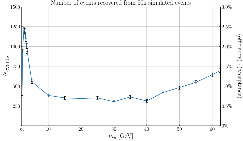
Figure 5.2: The number of OSSF0 events reconstructed from a simulation of 50 000 h \rightarrow aa decay events in MadGraph for sample masses between m_a = m_\tau and m_a = m_h/2 . The signal efficiency is then estimated by taking the fraction of such events.
