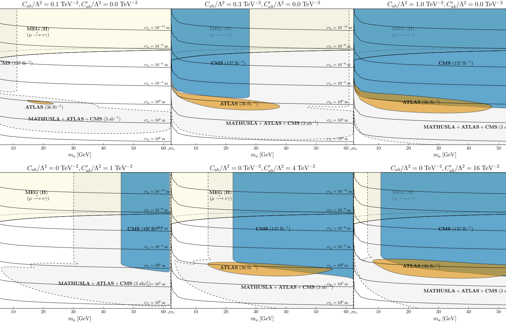
Figure 5.5: Combined limits on the leptophilic LFV ALP model considered in this section, over a range of different Higgs interaction couplings. Limits from LFV lepton decays are presented in yellow, with the leading limit coming from \mu \rightarrow e\gamma through an internal \tau . Limits from Higgs decays at CMS are shown in blue, and at ATLAS are shown in orange. Finally, combined projections from CMS, ATLAS, and MATHUSLA assuming \mathcal{L} = 3 \text{ ab}^{-1} of integrated luminosity are shown in gray.
