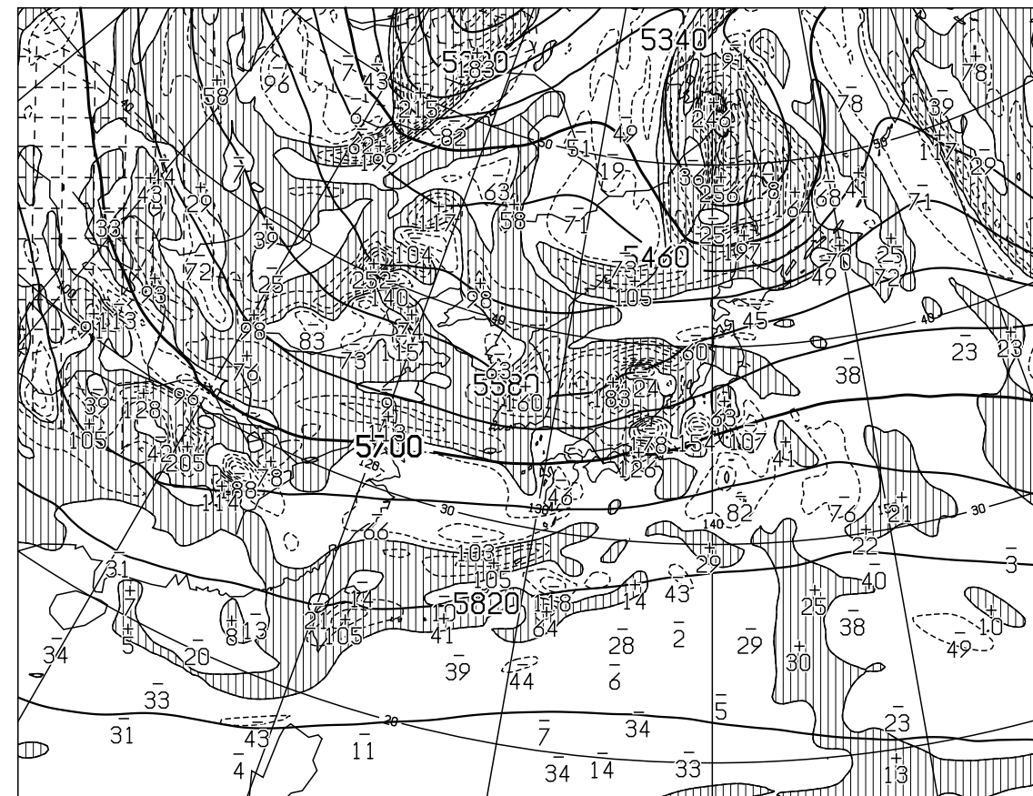
T=24 VALID 310000UTC HEIGHT(M),VORT(10 \times -6/SEC) AT 500hPa
