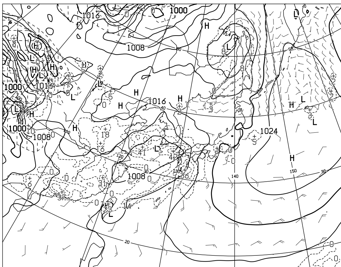
T=12 VALID 301200UTC SURFACE PRESS(hPa),PRECIP(MM) (00-12) WIND ARROW AT SURFACE
