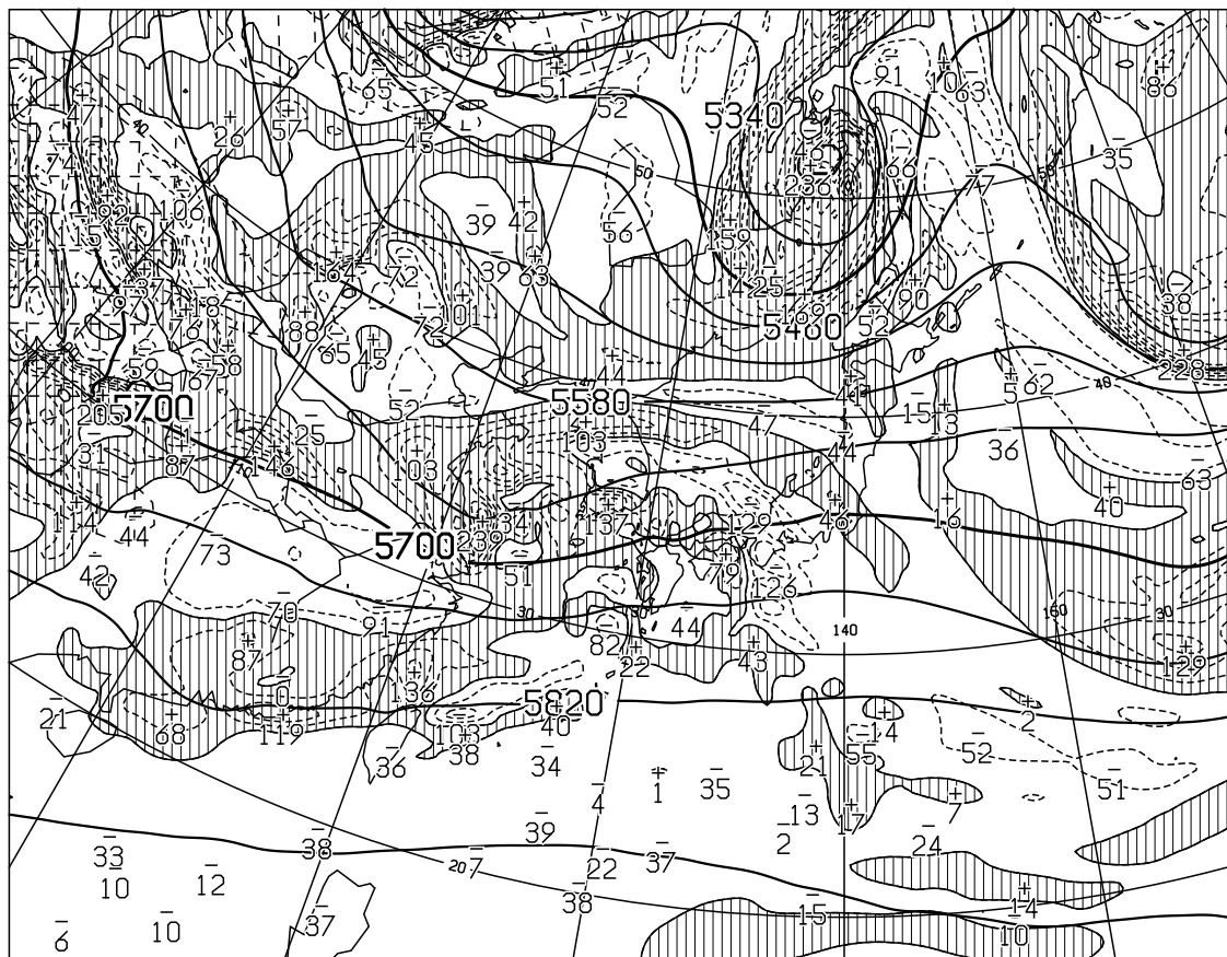
T=12 VALID 301200UTC HEIGHT(M),VORT(10 \times -6/SEC) AT 500hPa
