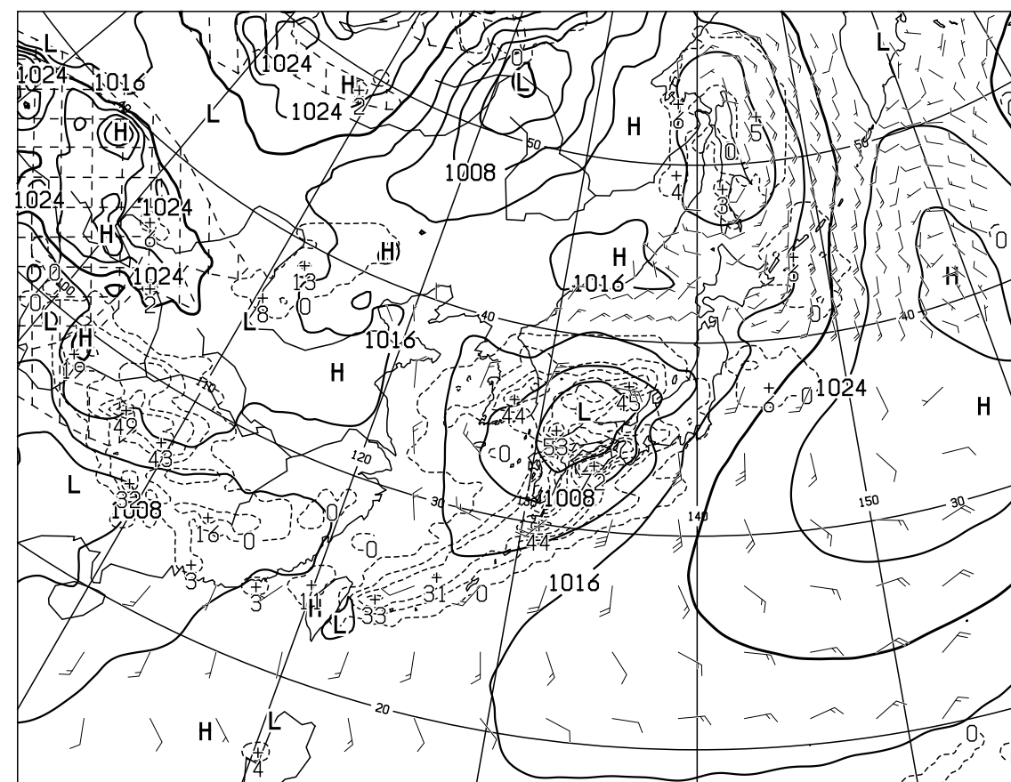
T=24 VALID 310000UTC SURFACE PRESS(hPa),PRECIP(MM) (12-24) WIND ARROW AT SURFACE
