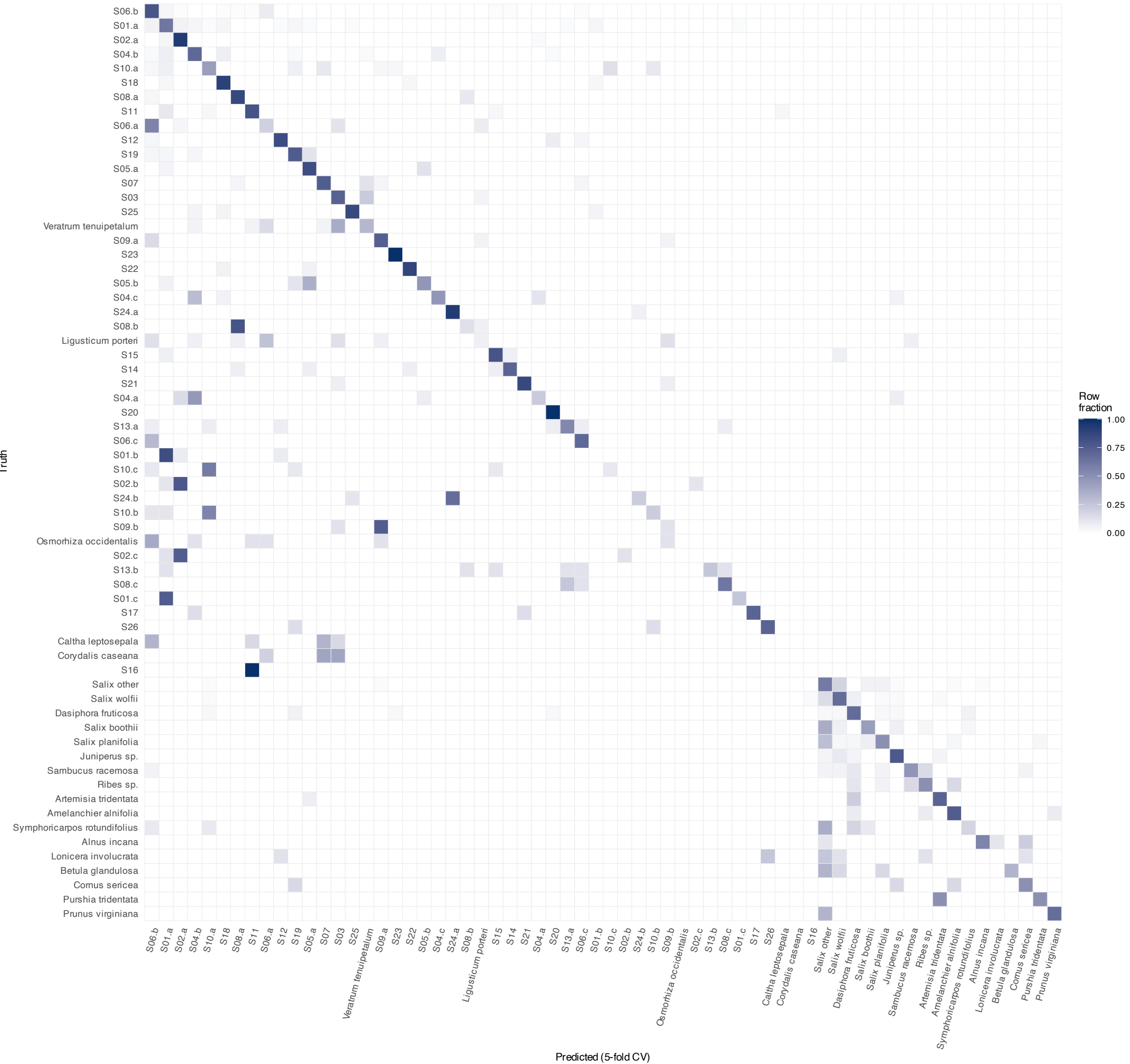
Joint meadow+shrub RF — row-normalized confusion matrix
