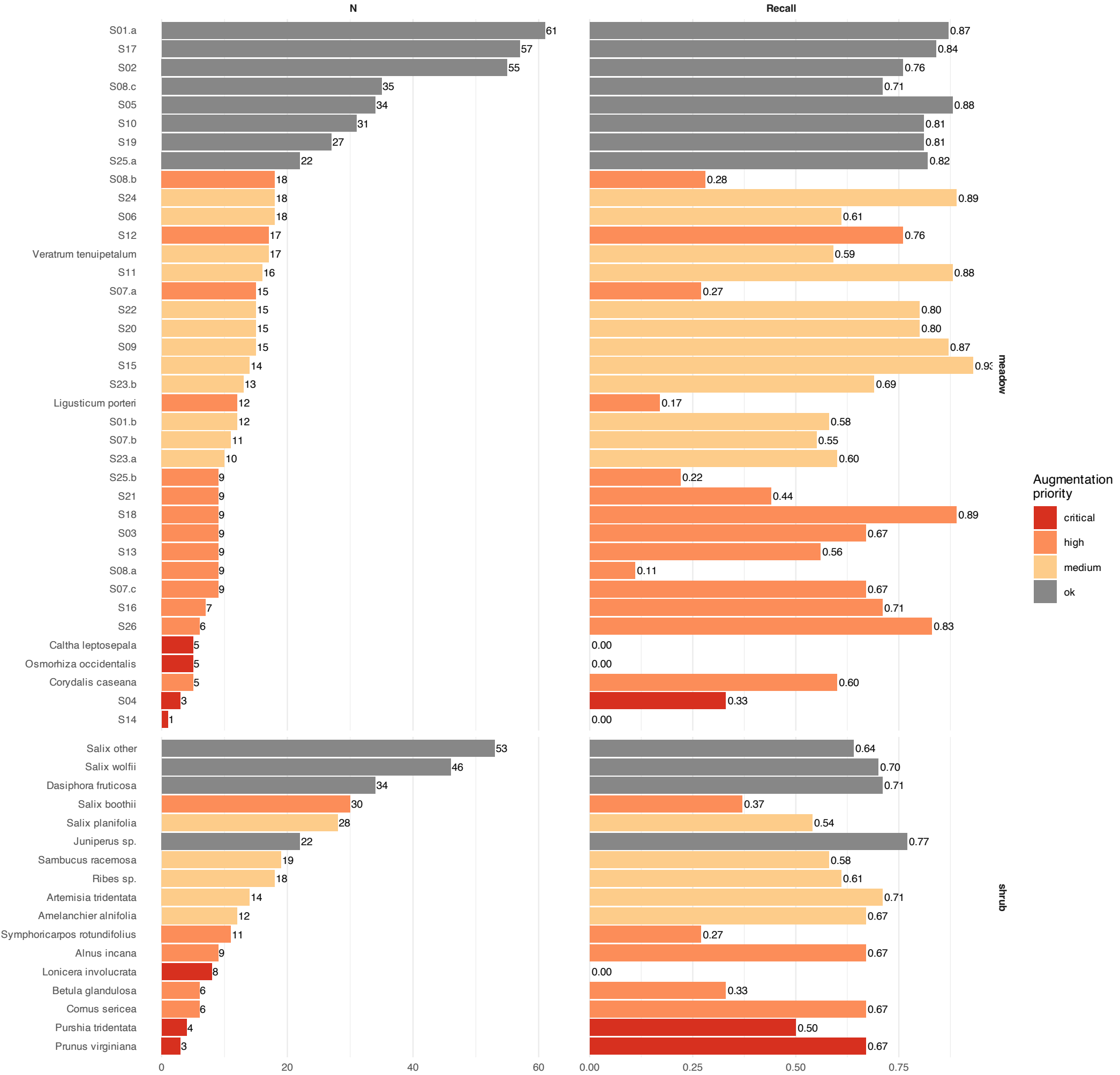
Joint meadow+shrub classifier — training N and CV recall per class Balanced 5-fold site-level CV; 858 sites, 47 classes
