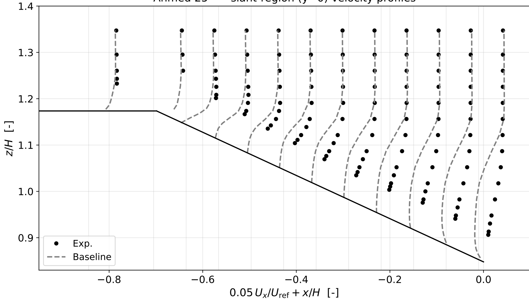
Ahmed 25° — slant-region ( y=0 ) velocity profiles
