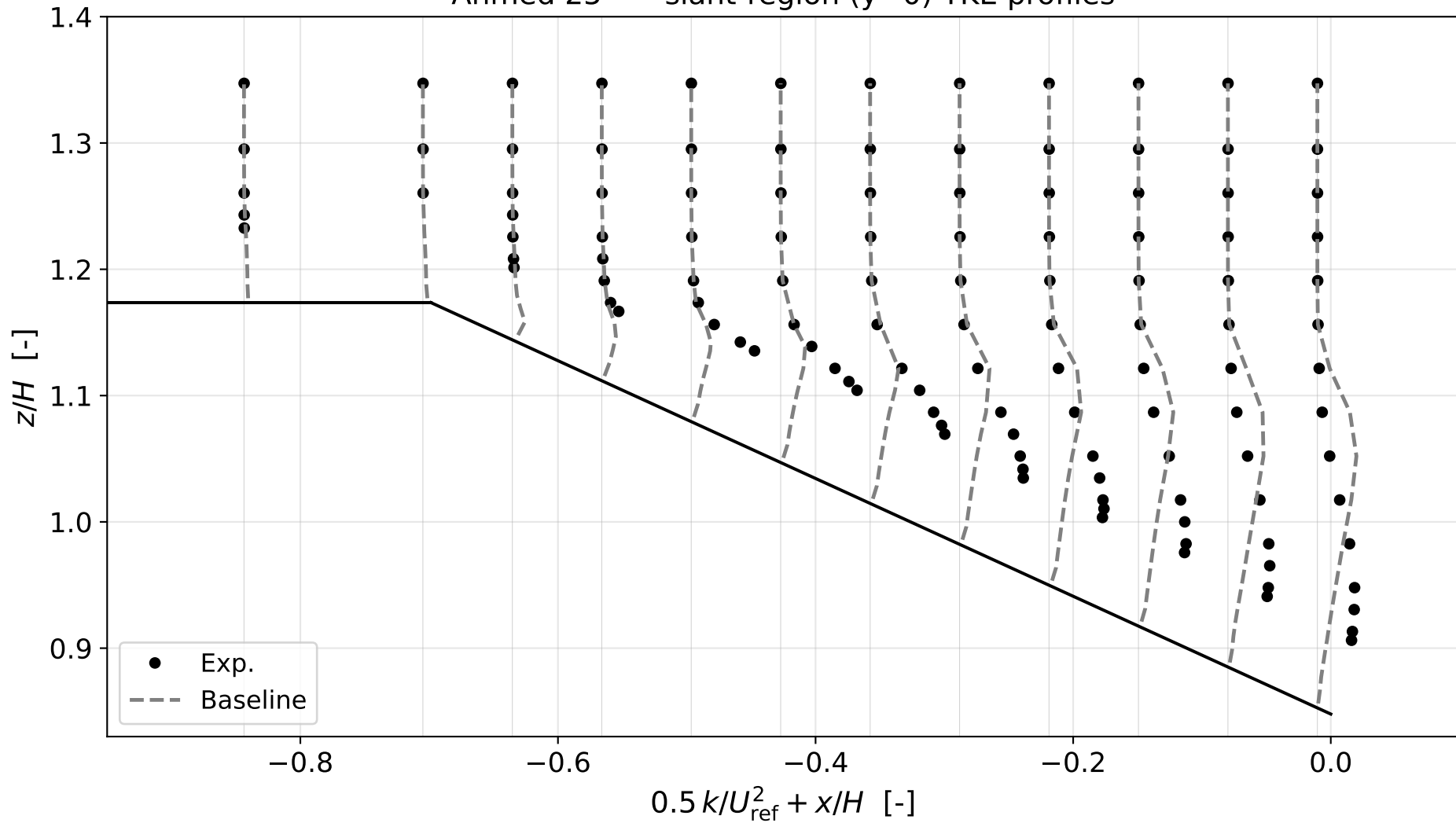
Ahmed 25° — slant-region ( y=0 ) TKE profiles
