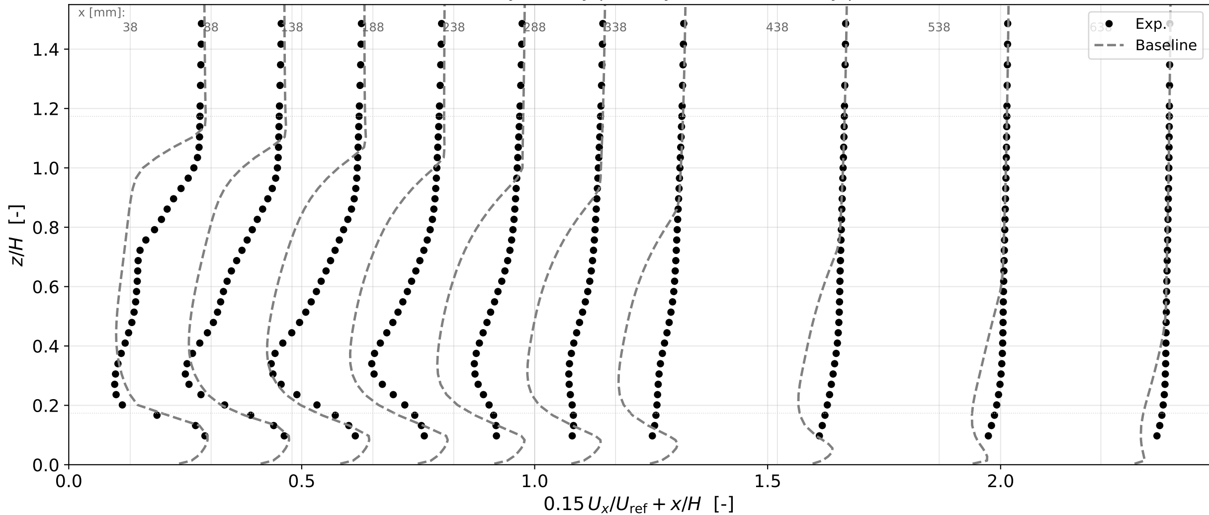
Ahmed 25° — symmetry-plane (y=0) wake velocity profiles
