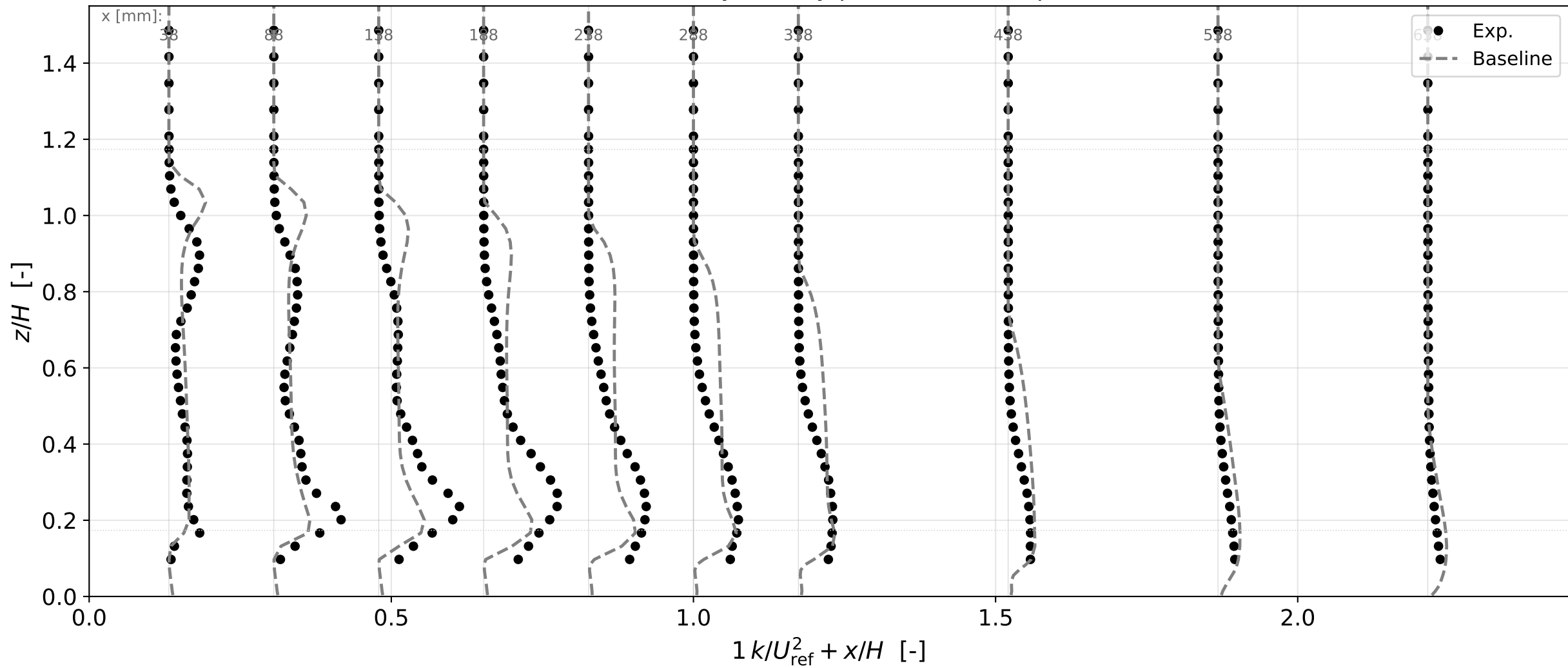
Ahmed 25° — symmetry-plane wake TKE profiles
