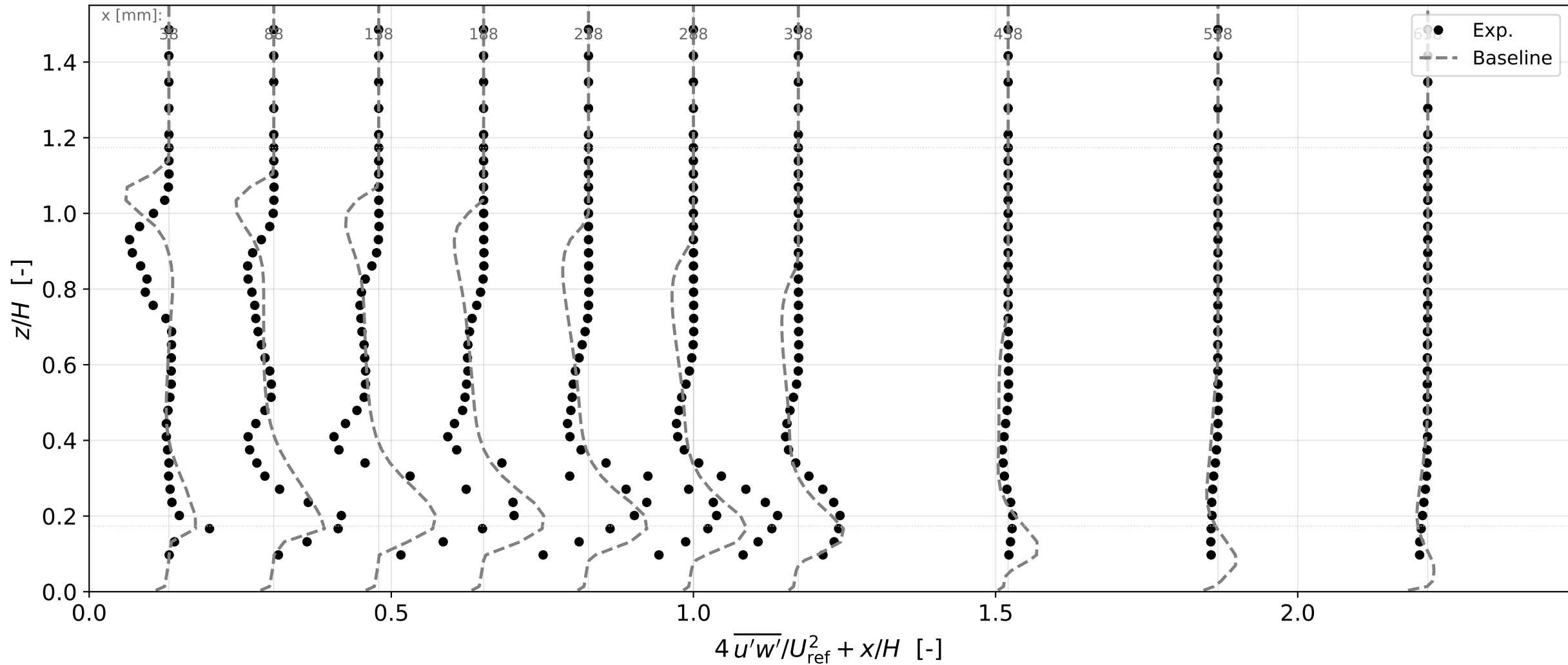
Ahmed 25° — symmetry-plane wake Reynolds shear stress
