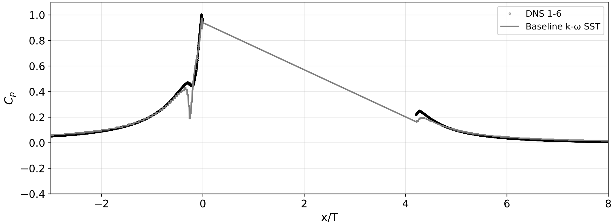
Bottom-wall centerline pressure ( z/T = 0 )
