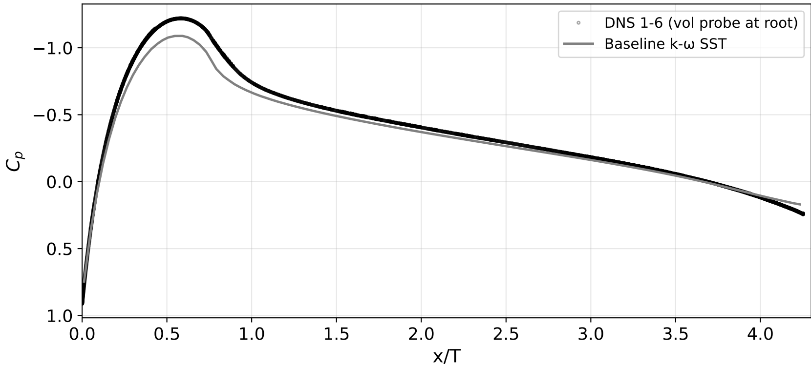
Wing root chord pressure (airfoil surface, y/T \rightarrow 0 )
