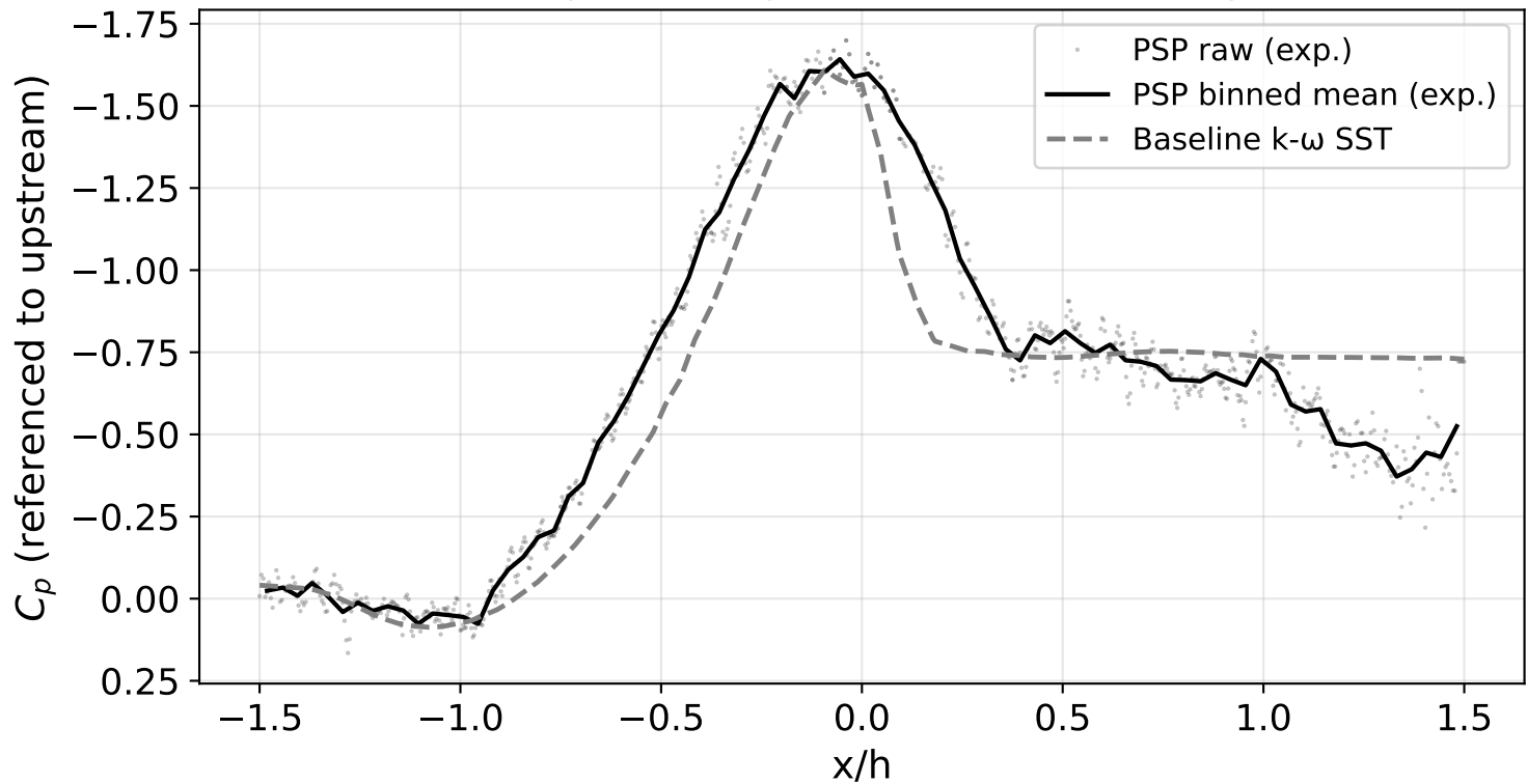
Faith Hill centerline wall pressure (upstream refs subtracted: exp=0.13, base=0.53)
