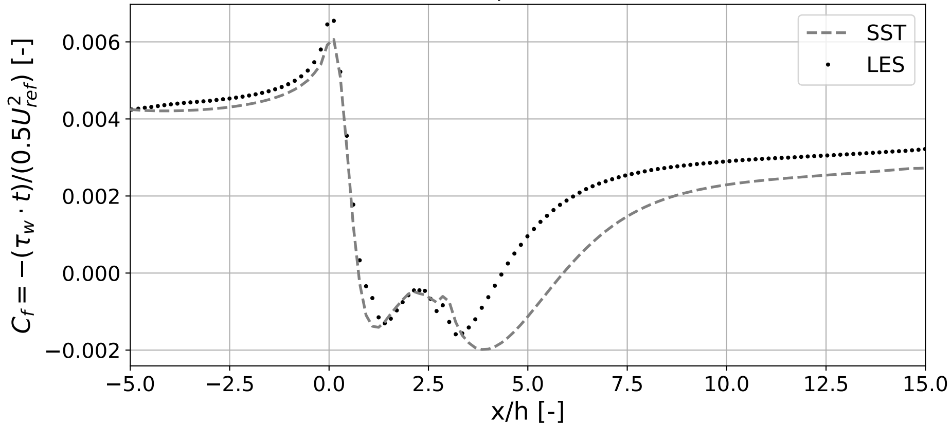
Bottom-Wall C_f Comparison ( U_{ref}(SST) = 1.00 )
