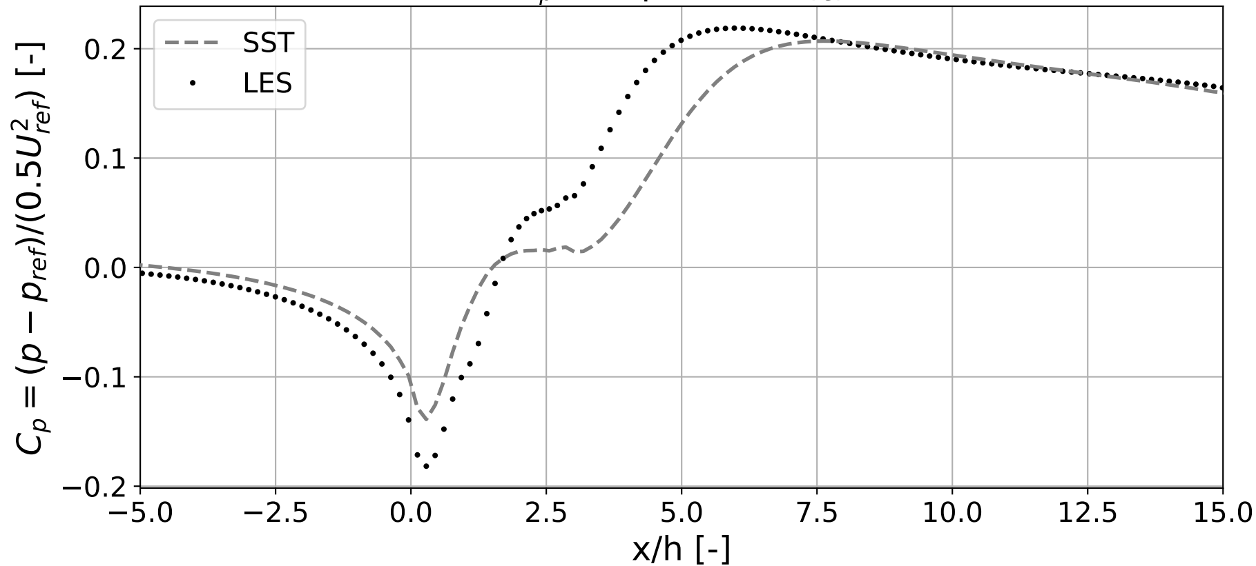
Bottom-Wall C_p Comparison ( U_{ref}(SST) = 1.00 )
