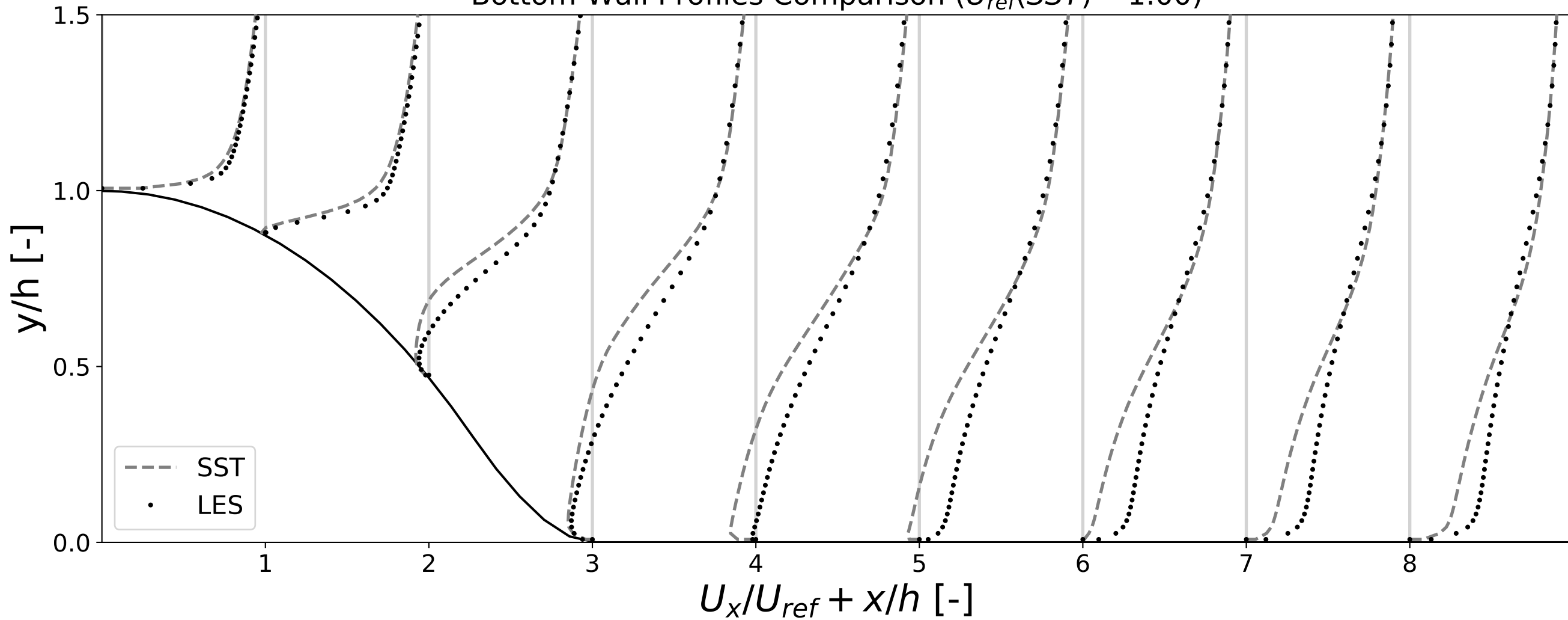
Bottom-Wall Profiles Comparison ( U_{ref}(SST) = 1.00 )
