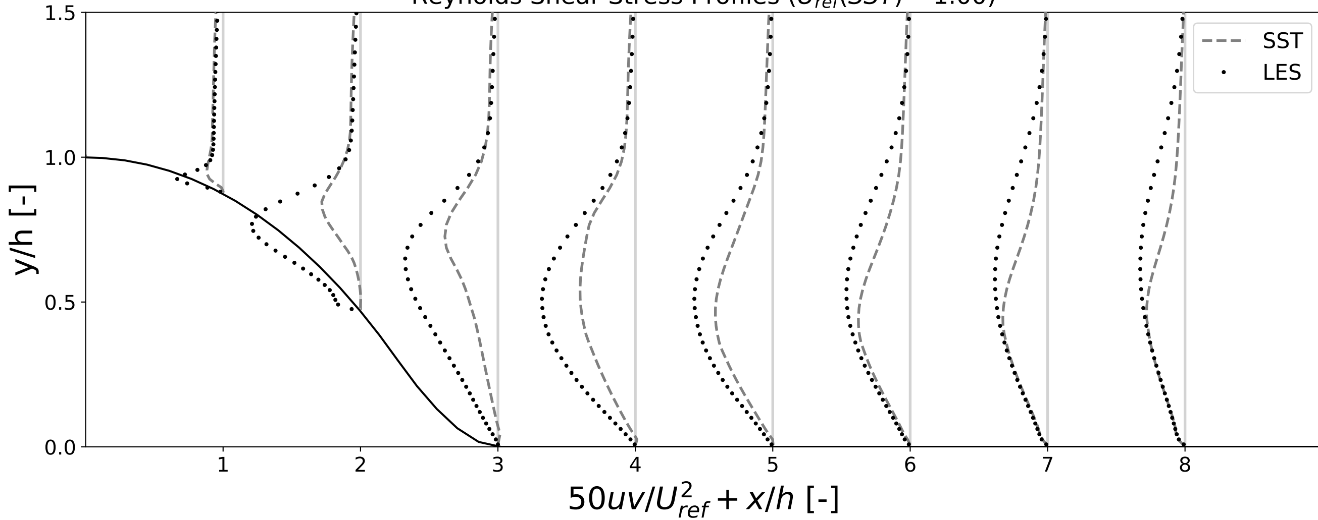
Reynolds Shear Stress Profiles ( U_{ref}(SST) = 1.00 )
