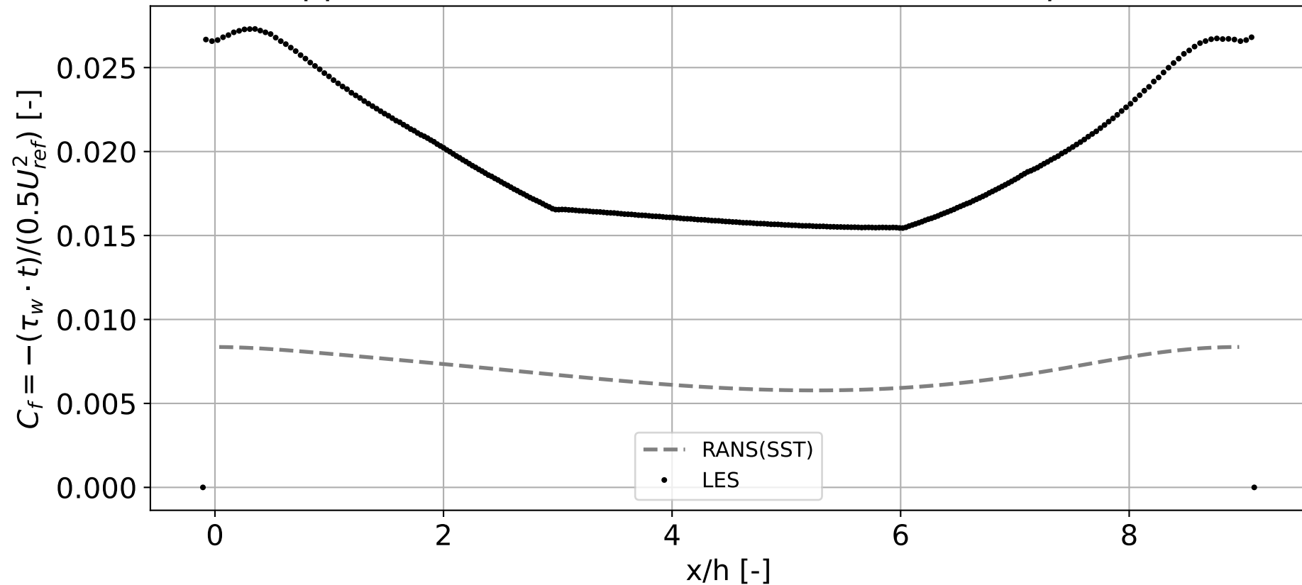
Upper Wall Skin-Friction Coefficient ( U_{ref} = 1, p_{ref} = 1 )
