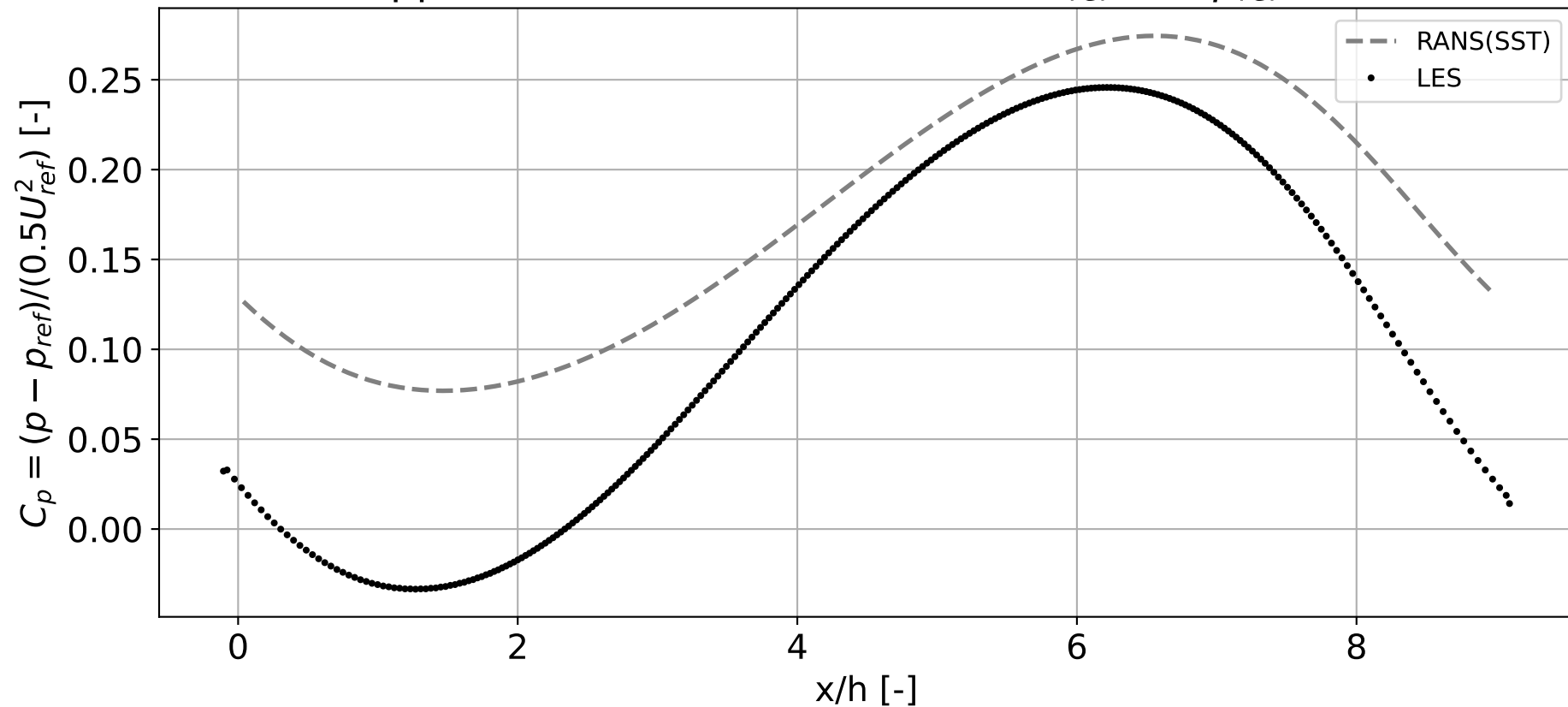
Upper Wall Pressure Coefficient ( U_{ref} = 1, p_{ref} = 1 )
