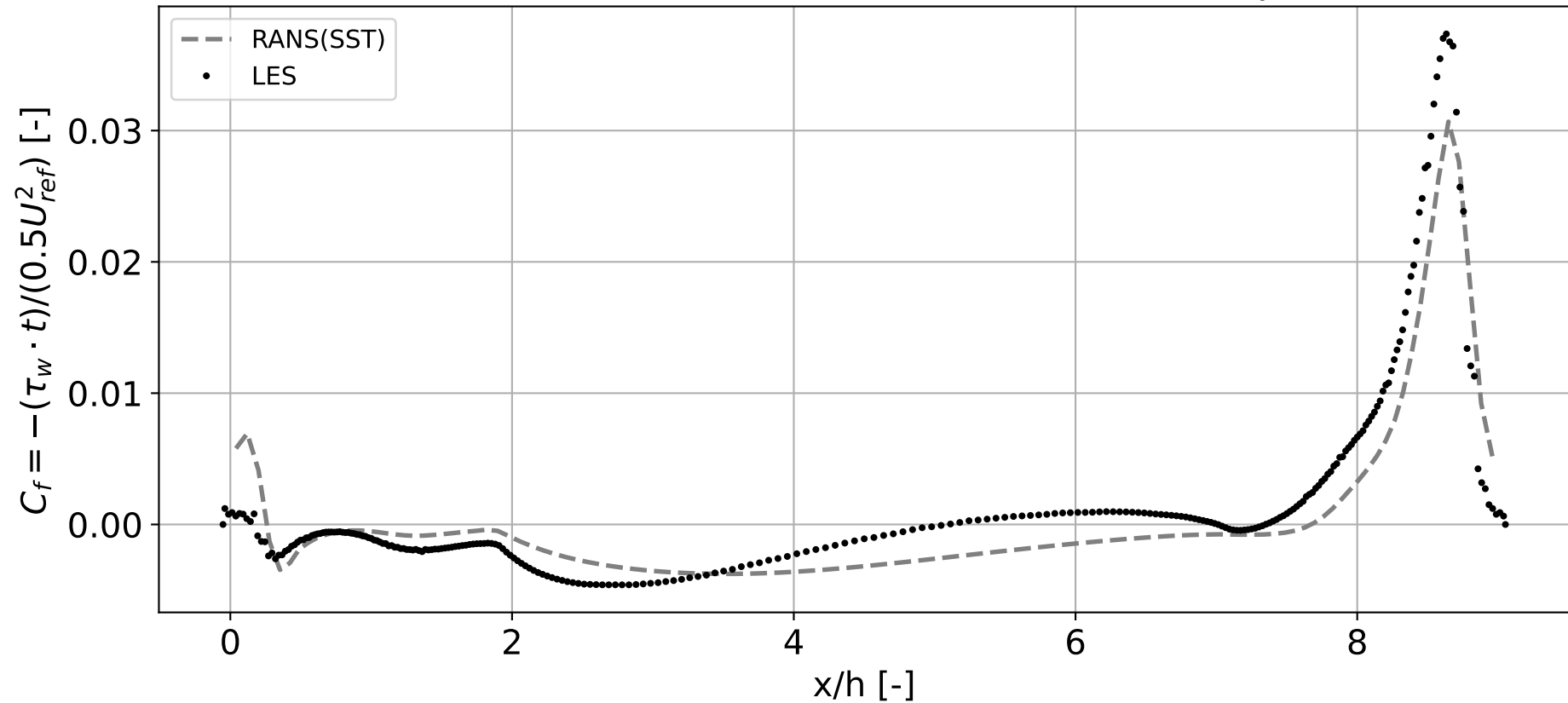
Bottom Wall Skin-Friction Coefficient ( U_{ref} = 1, p_{ref} = 1 )
