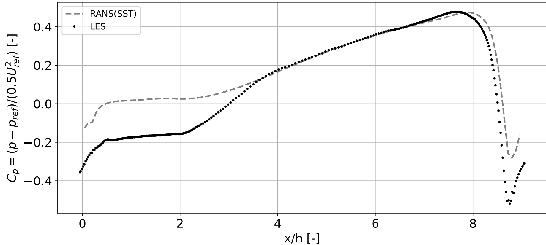
Bottom Wall Pressure Coefficient ( U_{ref} = 1, p_{ref} = 1 )
