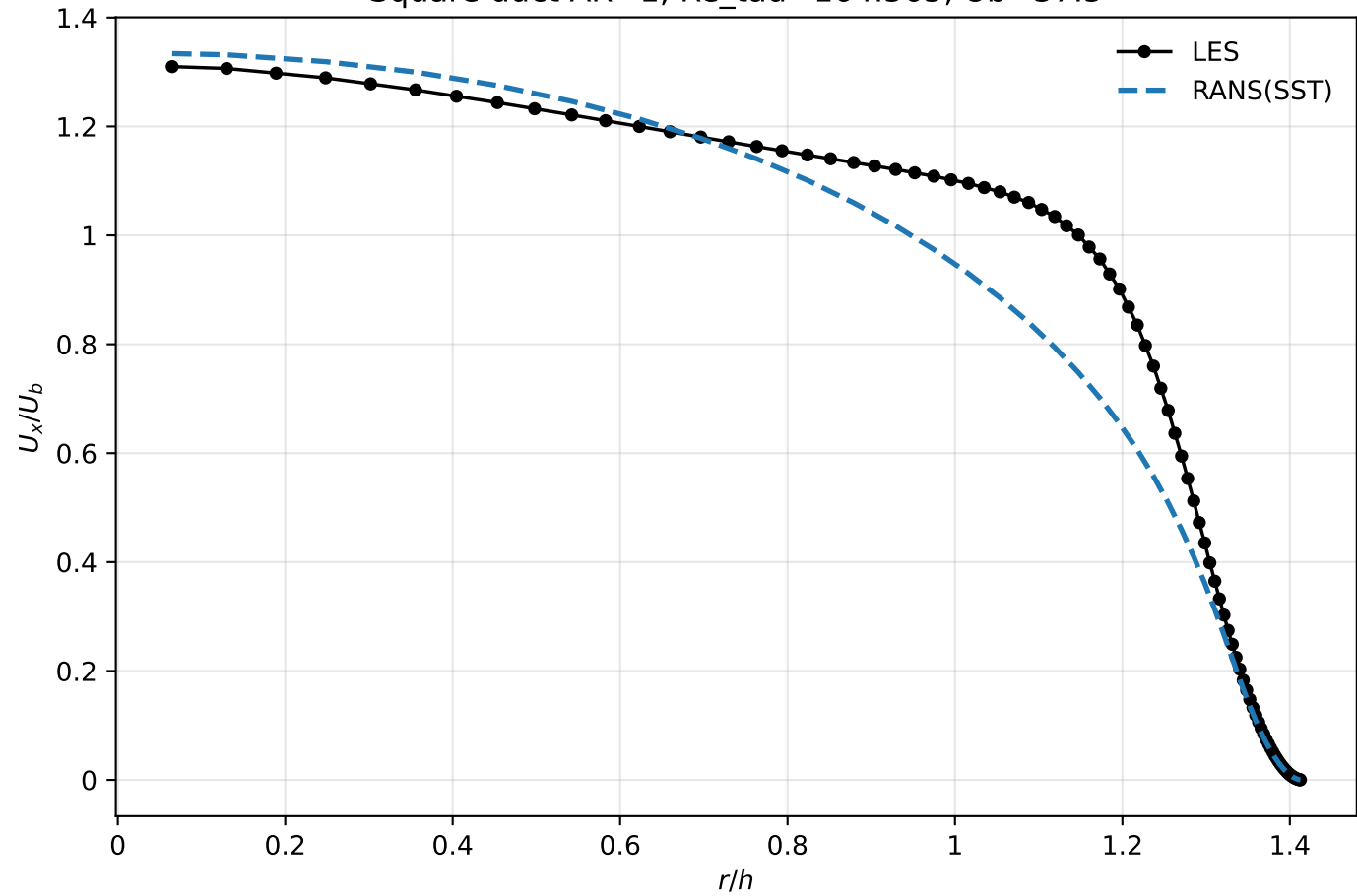
Square duct AR=1, Re_tau=164.565, U_b=37.5
