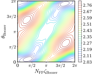
(b) Initial equilibrium |B| .
