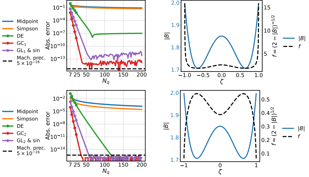
Figure 5: Convergence of quadratures for the well on the right is shown.
