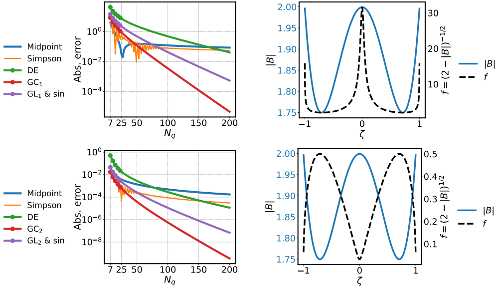
Figure 6: Convergence of quadratures for the well on the right is shown. In the top row, the integrand becomes nearly non-integrable as the parallel velocity nearly vanishes at \zeta = 0 . In either case, splitting the quadrature there recovers fast convergence.
