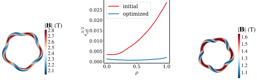
(a) Neoclassical transport optimization.
