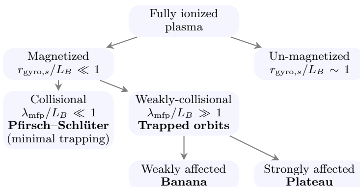
Figure 1: A schematic categorizing neoclassical transport is shown.
