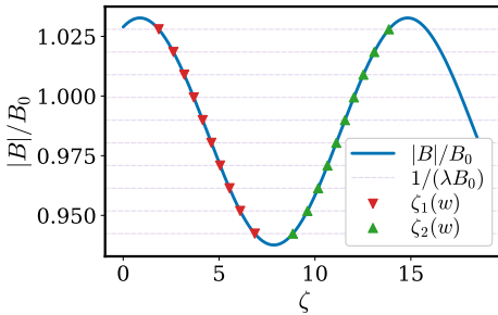
(a) For a pitch marked by a horizontal line, |v_{\parallel}| = 0 at the points marked by triangles.
