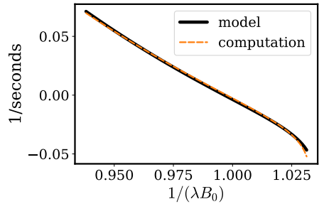
(b) The bounce-averaged binormal drift in the configuration in figure 11a is compared.
