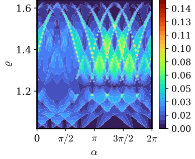
(e) Optimized bounce-averaged radial drifts.
