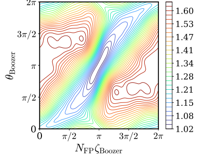
(c) Optimized equilibrium |B| .
