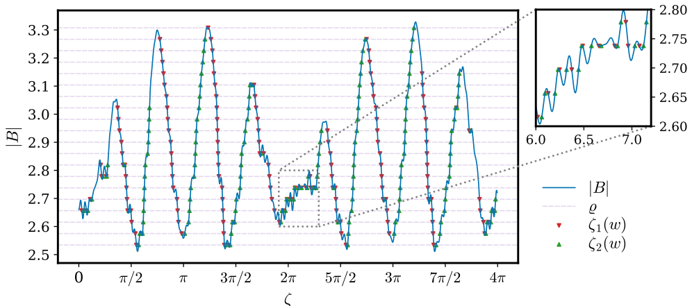
Figure 2: This figure shows bounce points within (\zeta_1, \zeta_2) = (0, 4\pi) on the field line (\psi, \alpha) = (1, 0) for a mesh of \rho values on a W7-X stellarator. For a given \rho marked by a horizontal line, |v_{\parallel}| = 0 at the bounce points marked by triangles. The plasma distribution vanishes in the hypograph of |B| .
