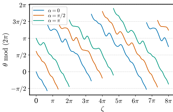
Figure 8: \theta on the plasma boundary of an NCSX stellarator with N_{FP} = 3 .
