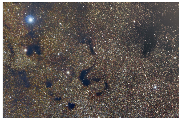
Snake nebula (B72 in Ophiuchus); image credit: Paolo Pinciaroli (Lebowsky) and www.astronomy.fm
