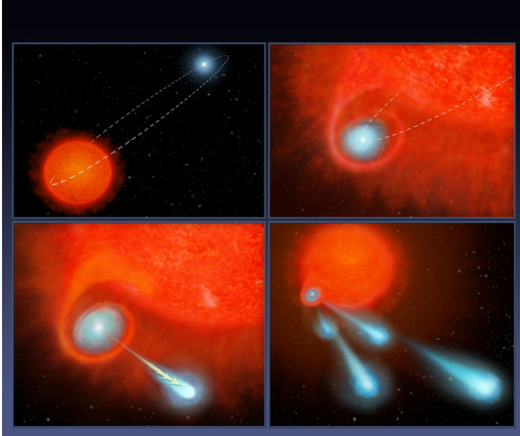
his four-panel graphic illustrates how the binary-star system V Hydrae is launching balls of plasma into space. Image credit: NASA/ESA/STScI
