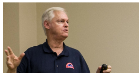
Bruce Kosaveach was our 2nd Guest Speaker of the evening. He told us all about the new additions to Lowell Observatory. Photo by Don.
