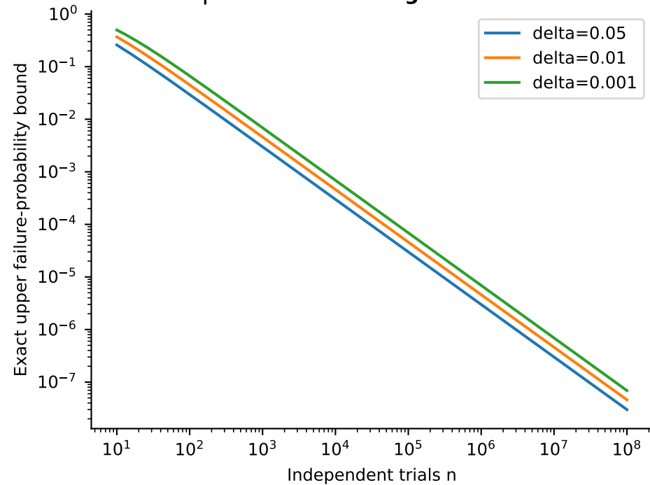
a | Zero-failure design calculation
