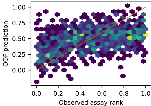
Sequence features + Ridge
