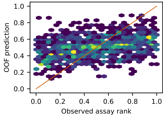
One-hot Ridge
