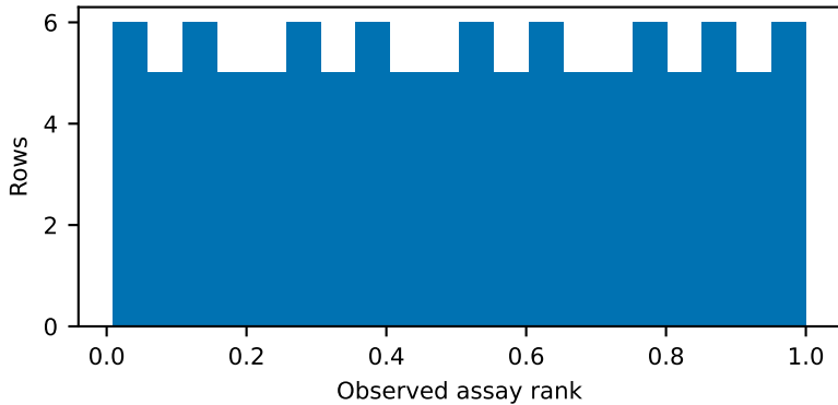
TADA1: supplied response distribution
