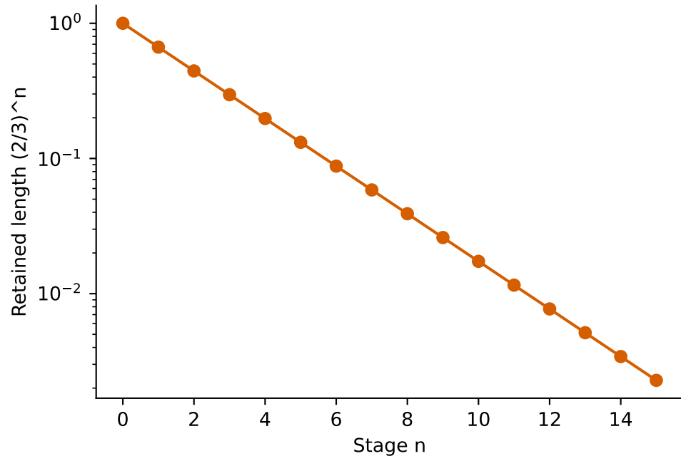
b | Finite-stage measure
