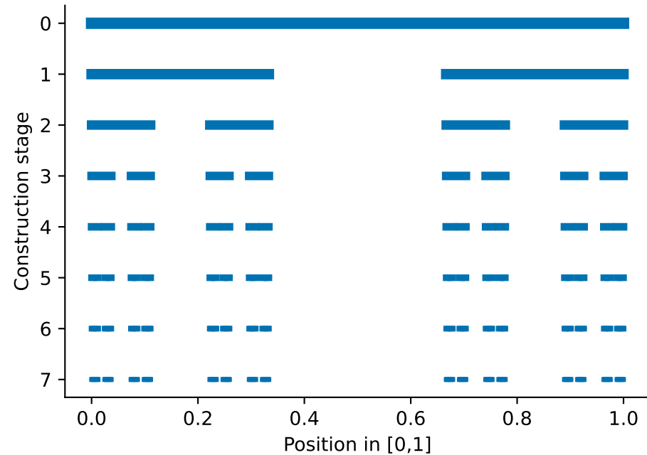
a | Cantor-stage intervals
